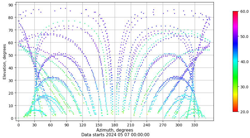
Azimuth-elevation plot for station TALR. Signal to Noise S1C Data file TALR00ESP_R_2024128.xtr
