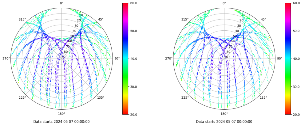
Skyplot for station TALR. Signal to Noise S1C Data file TALR00ESP_R_2024128.xtr Skyplot for station TALR. Signal to Noise S2C Data file TALR00ESP_R_2024128.xtr
