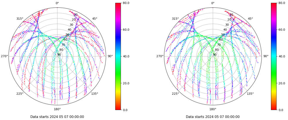
Skyplot for station TALR. Parameter M1C Data file TALR00ESP_R_2024128.xtr Skyplot for station TALR. Parameter M2C Data file TALR00ESP_R_2024128.xtr
