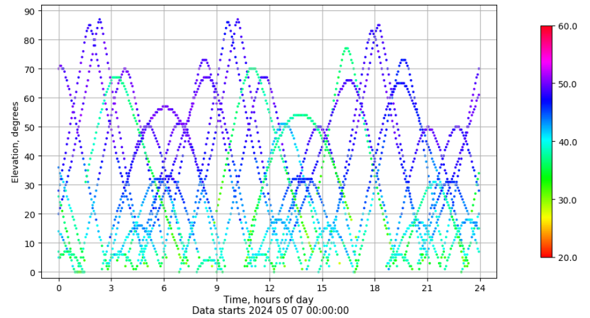
Time-elevation plot for station TALR. Signal to Noise S1C Data file TALR00ESP_R_2024128.xtr
