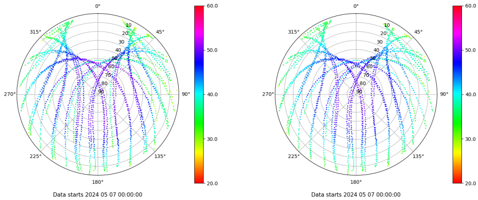
Skyplot for station SEV1. Signal to Noise S1C Data file SEV100ESP_R_2024128.xtr Skyplot for station SEV1. Signal to Noise S2C Data file SEV100ESP_R_2024128.xtr
