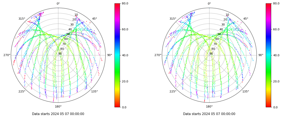
Skyplot for station SEV1. Parameter M1C Data file SEV100ESP_R_2024128.xtr Skyplot for station SEV1. Parameter M2C Data file SEV100ESP_R_2024128.xtr
