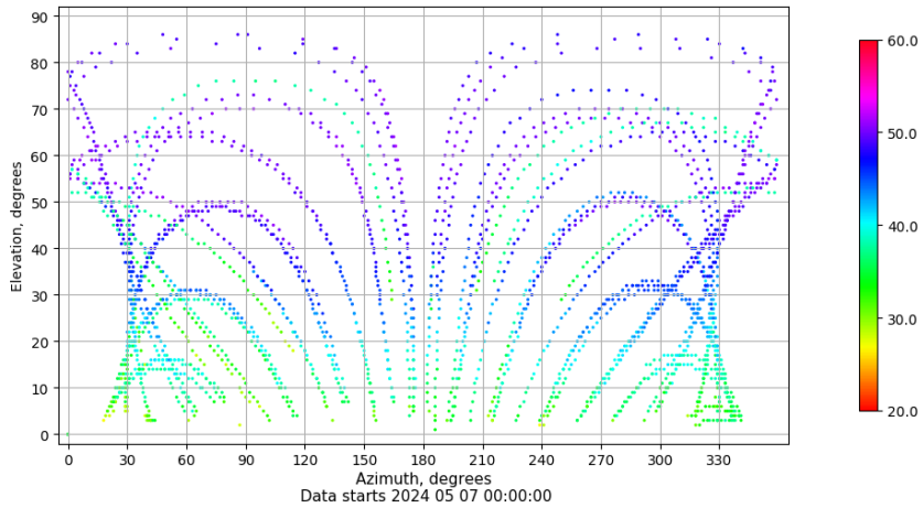
Azimuth-elevation plot for station SEV1. Signal to Noise S1C Data file SEV100ESP_R_2024128.xtr
