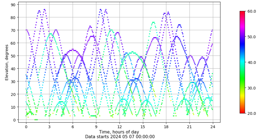
Time-elevation plot for station SEV1. Signal to Noise S1C Data file SEV100ESP_R_2024128.xtr
