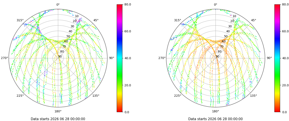
Skyplot for station SALA. Parameter M1C Data file SALA00ESP_R_2026179.xtr Skyplot for station SALA. Parameter M2P Data file SALA00ESP_R_2026179.xtr
