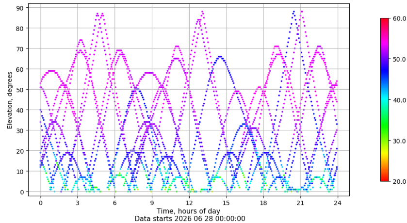
Time-elevation plot for station SALA. Signal to Noise S1C Data file SALA00ESP_R_2026179.xtr
