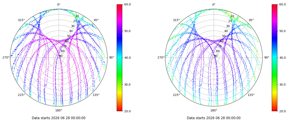
Skyplot for station SALA. Signal to Noise S1C Data file SALA00ESP_R_2026179.xtr Skyplot for station SALA. Signal to Noise S2P Data file SALA00ESP_R_2026179.xtr
