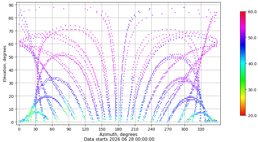
Azimuth-elevation plot for station SALA. Signal to Noise S1C Data file SALA00ESP_R_2026179.xtr
