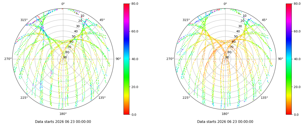
Skyplot for station SALA. Parameter M1C Data file SALA00ESP_R_2026174.xtr Skyplot for station SALA. Parameter M2P Data file SALA00ESP_R_2026174.xtr
