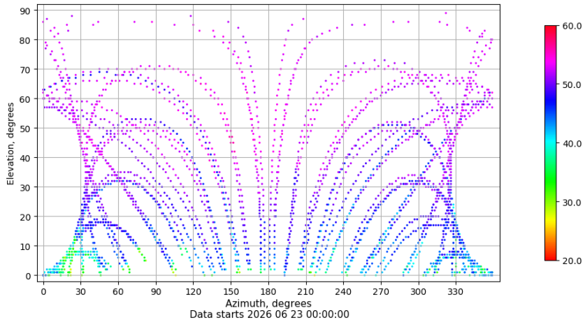
Azimuth-elevation plot for station SALA. Signal to Noise S1C Data file SALA00ESP_R_2026174.xtr
