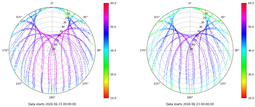
Skyplot for station SALA. Signal to Noise S1C Data file SALA00ESP_R_2026174.xtr Skyplot for station SALA. Signal to Noise S2P Data file SALA00ESP_R_2026174.xtr
