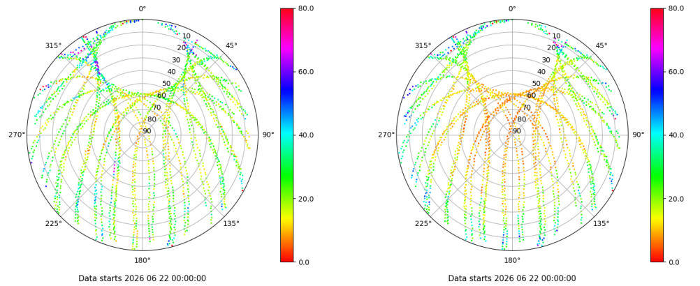
Skyplot for station SALA. Parameter M1C Data file SALA00ESP_R_2026173.xtr Skyplot for station SALA. Parameter M2P Data file SALA00ESP_R_2026173.xtr
