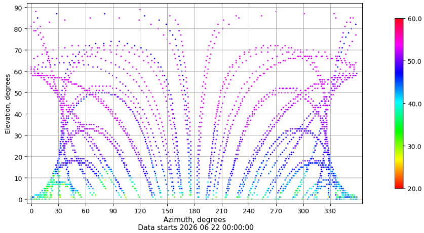
Azimuth-elevation plot for station SALA. Signal to Noise S1C Data file SALA00ESP_R_2026173.xtr
