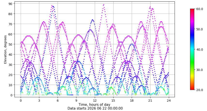
Time-elevation plot for station SALA. Signal to Noise S1C Data file SALA00ESP_R_2026173.xtr
