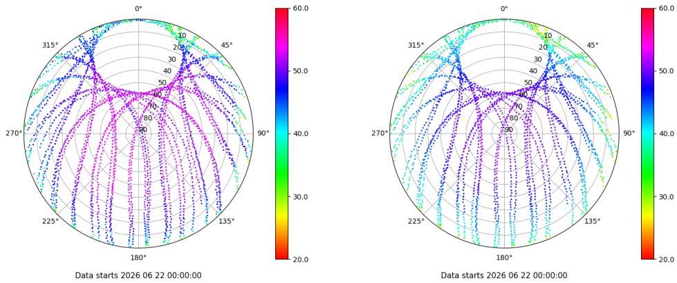
Skyplot for station SALA. Signal to Noise S1C Data file SALA00ESP_R_2026173.xtr Skyplot for station SALA. Signal to Noise S2P Data file SALA00ESP_R_2026173.xtr
