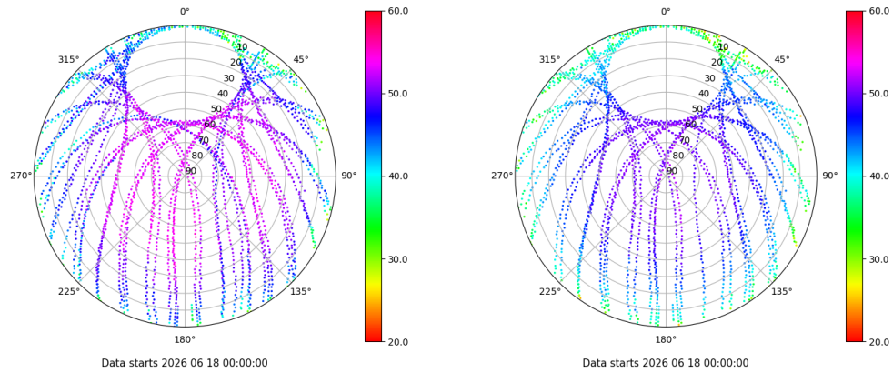
Skyplot for station SALA. Signal to Noise S1C Data file SALA00ESP_R_2026169.xtr Skyplot for station SALA. Signal to Noise S2P Data file SALA00ESP_R_2026169.xtr
