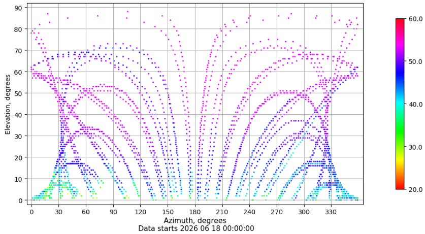
Azimuth-elevation plot for station SALA. Signal to Noise S1C Data file SALA00ESP_R_2026169.xtr
