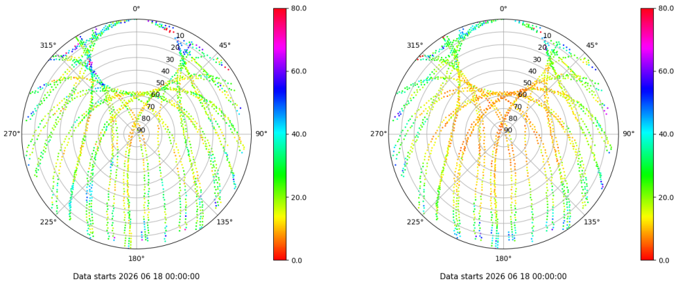
Skyplot for station SALA. Parameter M1C Data file SALA00ESP_R_2026169.xtr Skyplot for station SALA. Parameter M2P Data file SALA00ESP_R_2026169.xtr
