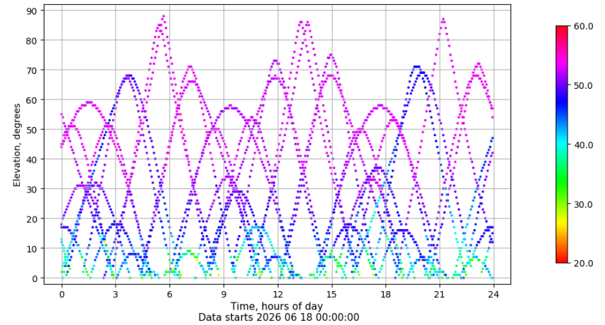
Time-elevation plot for station SALA. Signal to Noise S1C Data file SALA00ESP_R_2026169.xtr
