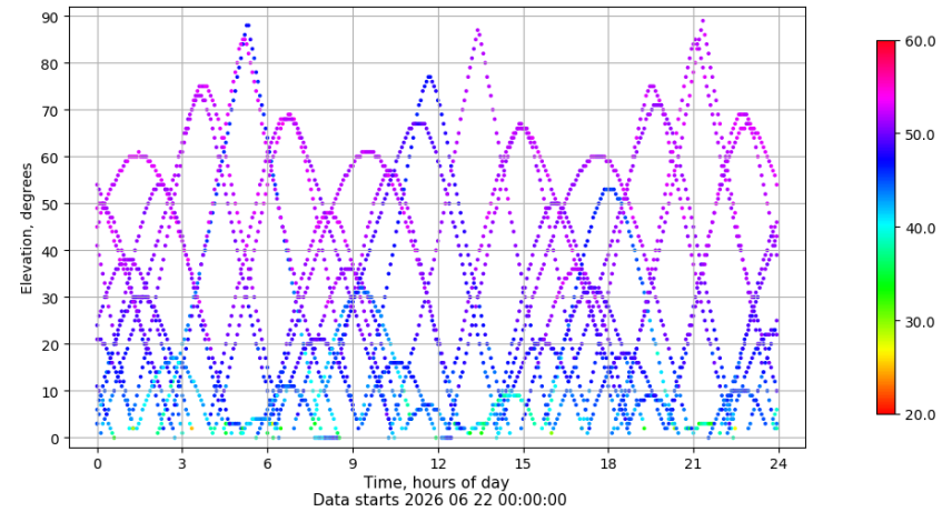
Time-elevation plot for station RIO1. Signal to Noise S1C Data file RIO100ESP_R_2026173.xtr
