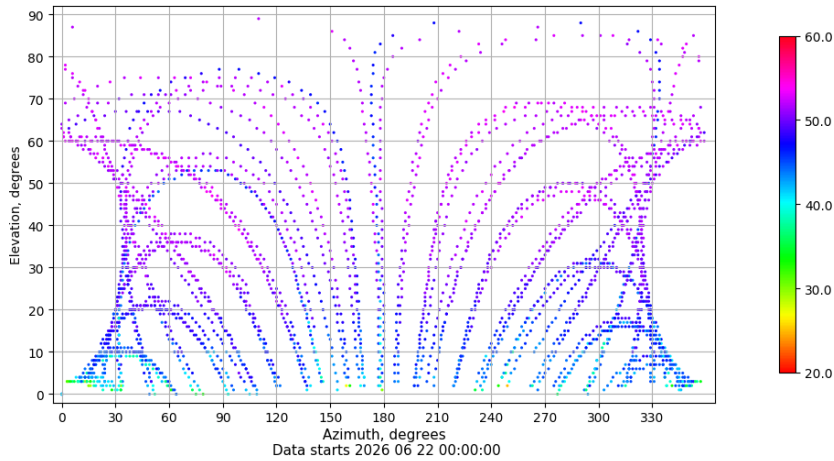
Azimuth-elevation plot for station RIO1. Signal to Noise S1C Data file RIO100ESP_R_2026173.xtr
