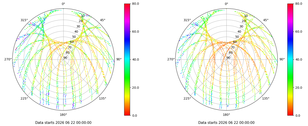
Skyplot for station RIO1. Parameter M1C Data file RIO100ESP_R_2026173.xtr Skyplot for station RIO1. Parameter M2P Data file RIO100ESP_R_2026173.xtr
