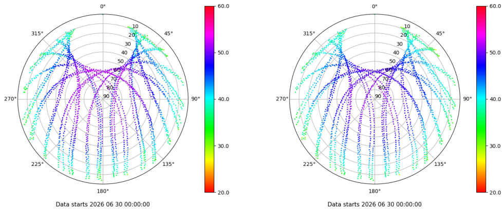
Skyplot for station PUIG. Signal to Noise S1C Data file PUIG00ESP_R_2026181.xtr Skyplot for station PUIG. Signal to Noise S2C Data file PUIG00ESP_R_2026181.xtr
