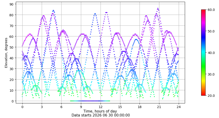
Time-elevation plot for station PUIG. Signal to Noise S1C Data file PUIG00ESP_R_2026181.xtr
