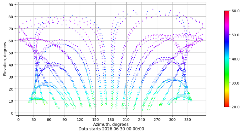
Azimuth-elevation plot for station PUIG. Signal to Noise S1C Data file PUIG00ESP_R_2026181.xtr
