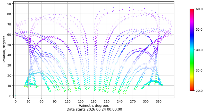
Azimuth-elevation plot for station PUIG. Signal to Noise S1C Data file PUIG00ESP_R_2026175.xtr
