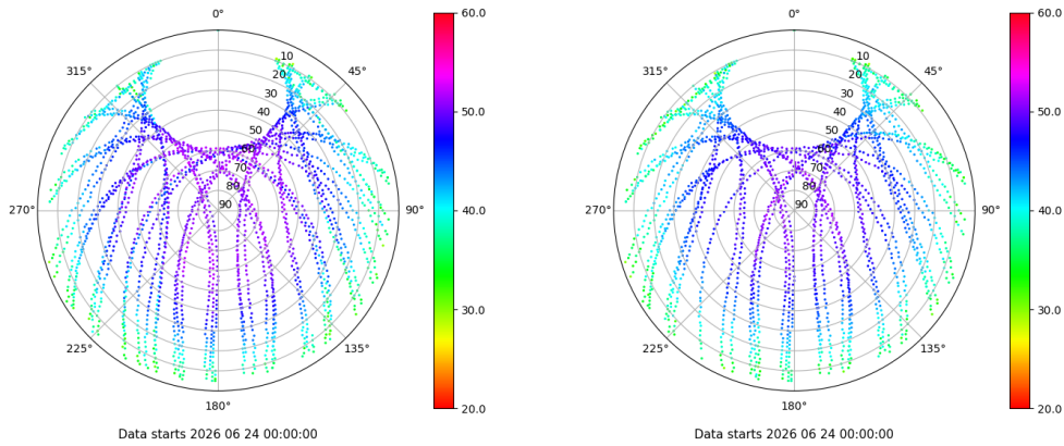
Skyplot for station PUIG. Signal to Noise S1C Data file PUIG00ESP_R_2026175.xtr Skyplot for station PUIG. Signal to Noise S2C Data file PUIG00ESP_R_2026175.xtr
