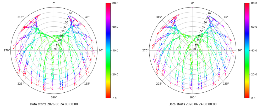
Skyplot for station PUIG. Parameter M1C Data file PUIG00ESP_R_2026175.xtr Skyplot for station PUIG. Parameter M2C Data file PUIG00ESP_R_2026175.xtr
