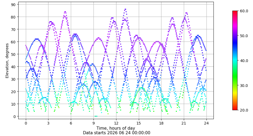
Time-elevation plot for station PUIG. Signal to Noise S1C Data file PUIG00ESP_R_2026175.xtr
