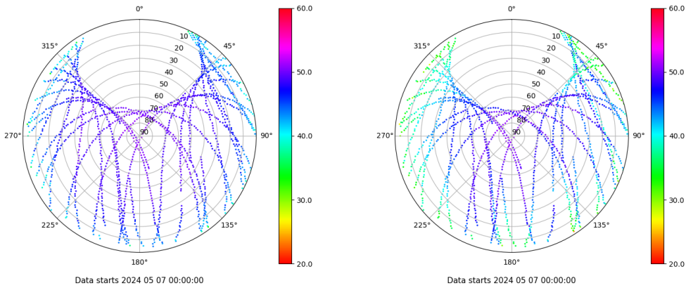
Skyplot for station PENI. Signal to Noise S1C Data file PENI00ESP_R_2024128.xtr Skyplot for station PENI. Signal to Noise S2W Data file PENI00ESP_R_2024128.xtr
