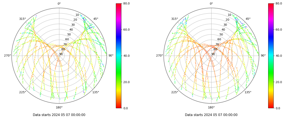
Skyplot for station PENI. Parameter M1C Data file PENI00ESP_R_2024128.xtr Skyplot for station PENI. Parameter M2W Data file PENI00ESP_R_2024128.xtr
