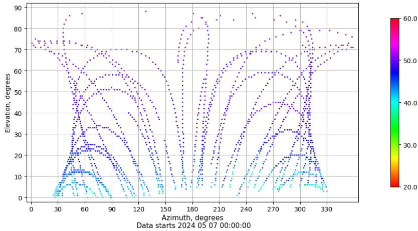
Azimuth-elevation plot for station PENI. Signal to Noise S1C Data file PENI00ESP_R_2024128.xtr
