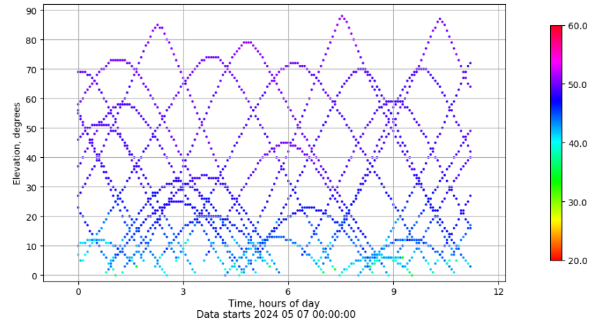
Time-elevation plot for station PENI. Signal to Noise S1C Data file PENI00ESP_R_2024128.xtr
