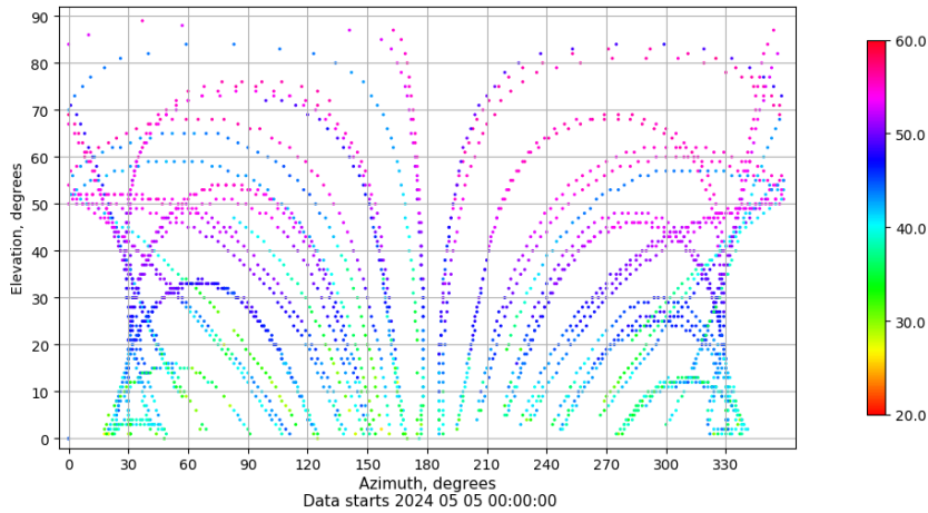
Azimuth-elevation plot for station MLLL. Signal to Noise S1C Data file MLLL00ESP_R_2024126.xtr
