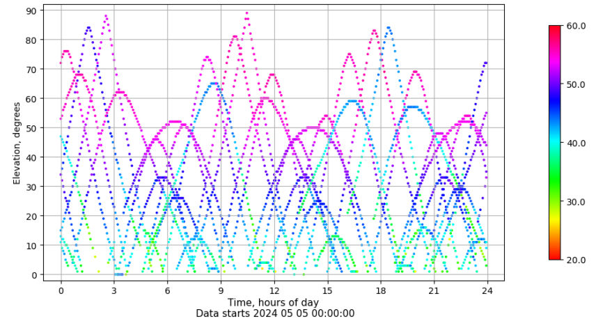
Time-elevation plot for station MLLL. Signal to Noise S1C Data file MLLL00ESP_R_2024126.xtr
