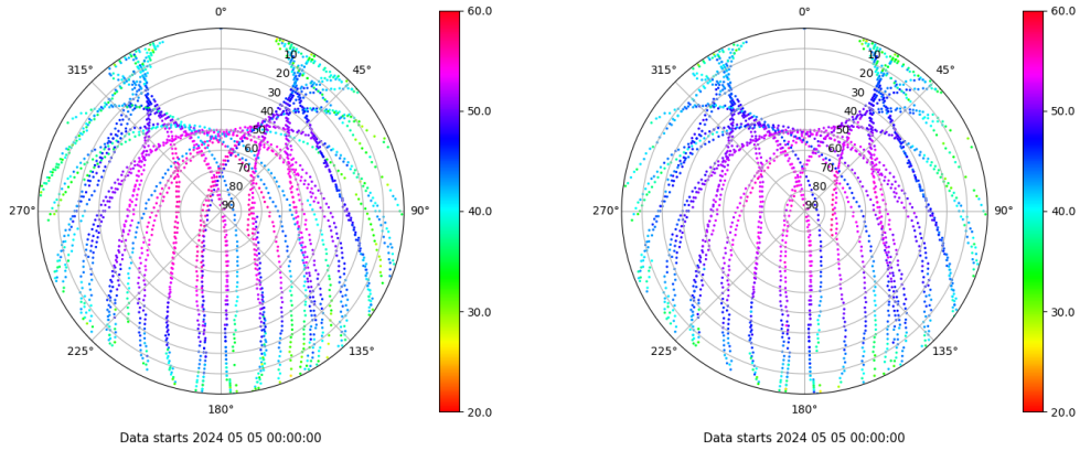
Skyplot for station MLLL. Signal to Noise S1C Data file MLLL00ESP_R_2024126.xtr Skyplot for station MLLL. Signal to Noise S2C Data file MLLL00ESP_R_2024126.xtr
