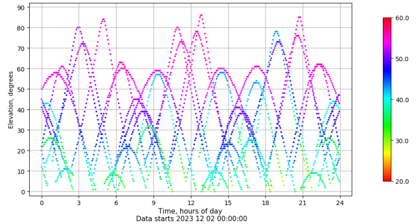
Time-elevation plot for station MALL. Signal to Noise S1C Data file MALL00ESP_R_2023336.xtr
