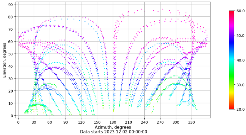
Azimuth-elevation plot for station MALL. Signal to Noise S1C Data file MALL00ESP_R_2023336.xtr
