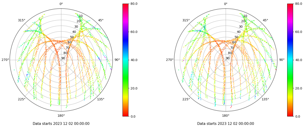
Skyplot for station MALL. Parameter M1C Data file MALL00ESP_R_2023336.xtr Skyplot for station MALL. Parameter M2C Data file MALL00ESP_R_2023336.xtr
