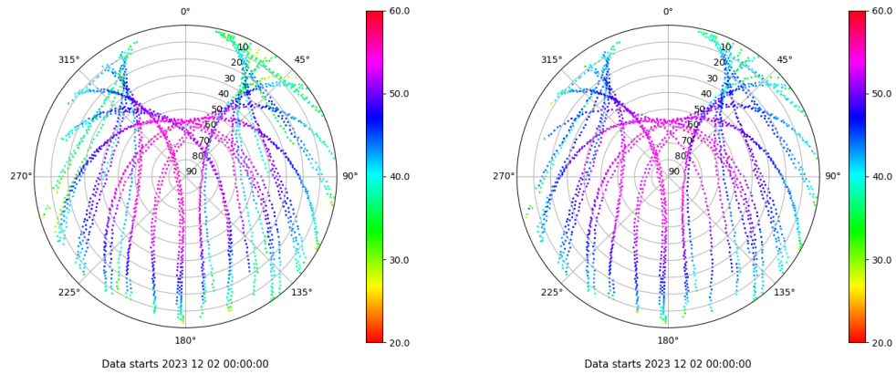
Skyplot for station MALL. Signal to Noise S1C Data file MALL00ESP_R_2023336.xtr Skyplot for station MALL. Signal to Noise S2C Data file MALL00ESP_R_2023336.xtr
