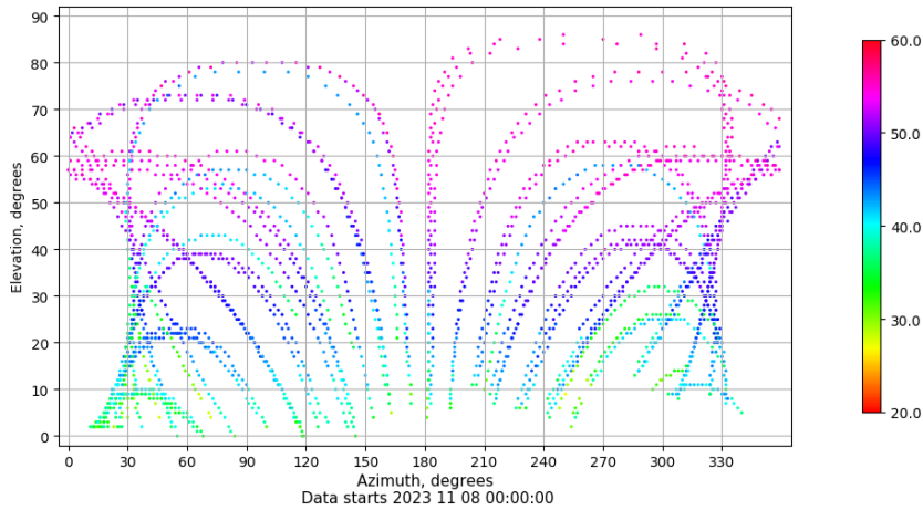
Azimuth-elevation plot for station MALL. Signal to Noise S1C Data file MALL00ESP_R_2023312.xtr
