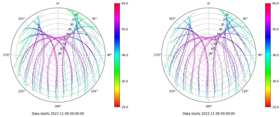
Skyplot for station MALL. Signal to Noise S1C Data file MALL00ESP_R_2023312.xtr Skyplot for station MALL. Signal to Noise S2C Data file MALL00ESP_R_2023312.xtr
