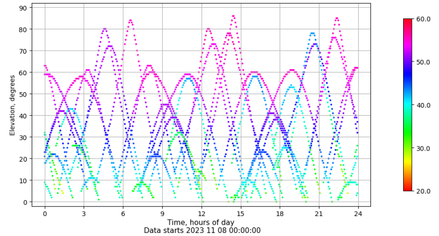
Time-elevation plot for station MALL. Signal to Noise S1C Data file MALL00ESP_R_2023312.xtr
