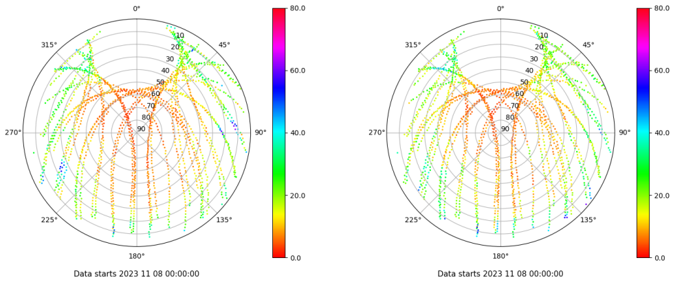
Skyplot for station MALL. Parameter M1C Data file MALL00ESP_R_2023312.xtr Skyplot for station MALL. Parameter M2C Data file MALL00ESP_R_2023312.xtr
