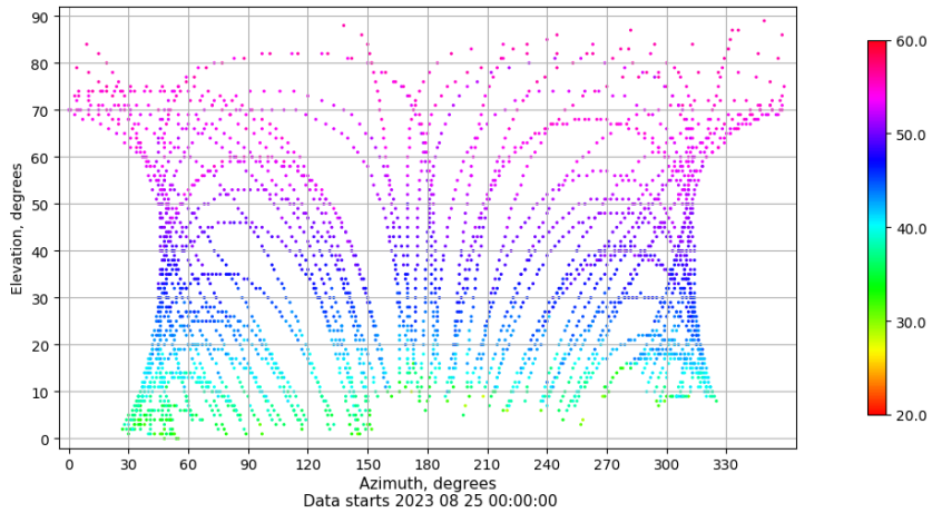
Azimuth-elevation plot for station MALL. Signal to Noise S1C Data file MALL00ESP_R_2023237.xtr
