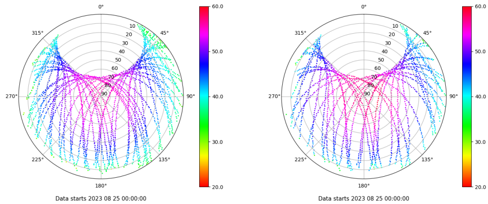
Skyplot for station MALL. Signal to Noise S1C Data file MALL00ESP_R_2023237.xtr Skyplot for station MALL. Signal to Noise S2S Data file MALL00ESP_R_2023237.xtr
