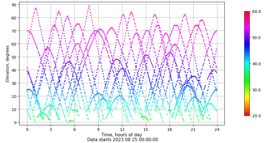
Time-elevation plot for station MALL. Signal to Noise S1C Data file MALL00ESP_R_2023237.xtr
