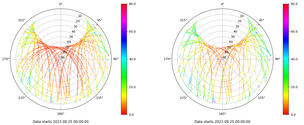
Skyplot for station MALL. Parameter M1C Data file MALL00ESP_R_2023237.xtr Skyplot for station MALL. Parameter M2S Data file MALL00ESP_R_2023237.xtr
