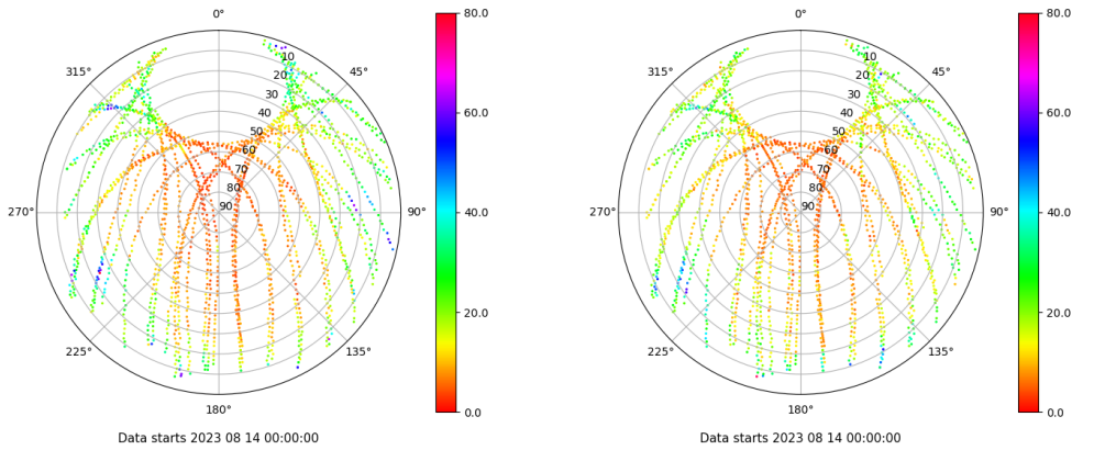
Skyplot for station MALL. Parameter M1C Data file MALL00ESP_R_2023226.xtr Skyplot for station MALL. Parameter M2C Data file MALL00ESP_R_2023226.xtr
