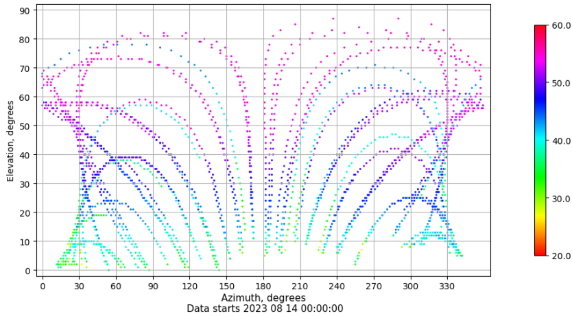
Azimuth-elevation plot for station MALL. Signal to Noise S1C Data file MALL00ESP_R_2023226.xtr
