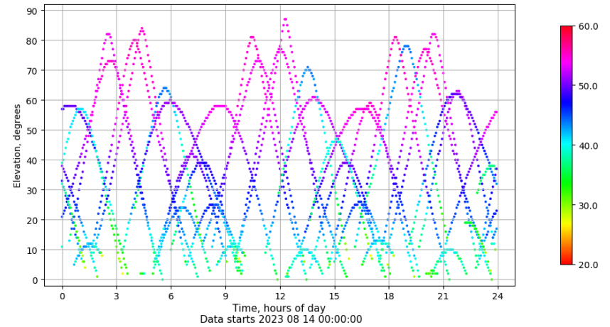
Time-elevation plot for station MALL. Signal to Noise S1C Data file MALL00ESP_R_2023226.xtr
