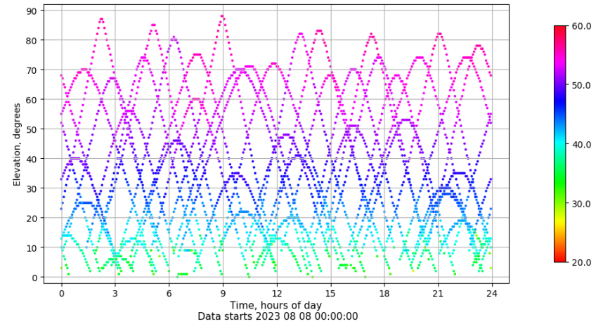
Time-elevation plot for station MALL. Signal to Noise S1C Data file MALL00ESP_R_2023220.xtr
