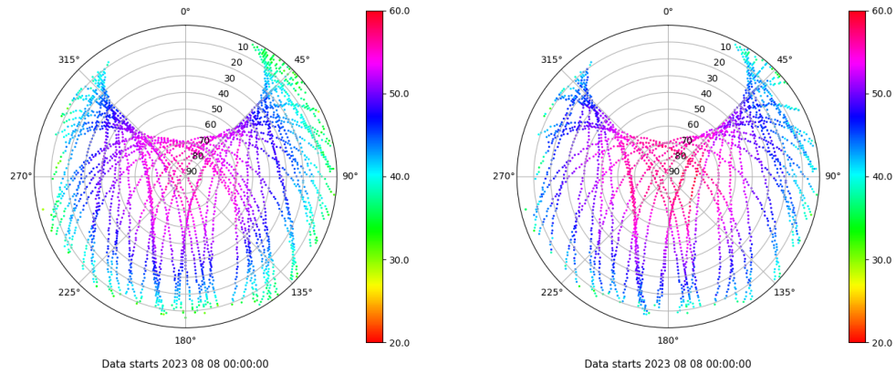
Skyplot for station MALL. Signal to Noise S1C Data file MALL00ESP_R_2023220.xtr Skyplot for station MALL. Signal to Noise S2S Data file MALL00ESP_R_2023220.xtr
