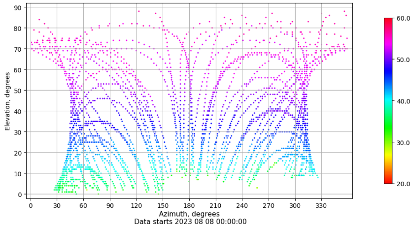
Azimuth-elevation plot for station MALL. Signal to Noise S1C Data file MALL00ESP_R_2023220.xtr
