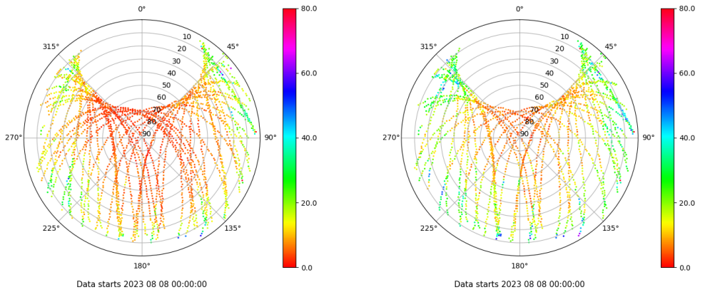
Skyplot for station MALL. Parameter M1C Data file MALL00ESP_R_2023220.xtr Skyplot for station MALL. Parameter M2S Data file MALL00ESP_R_2023220.xtr
