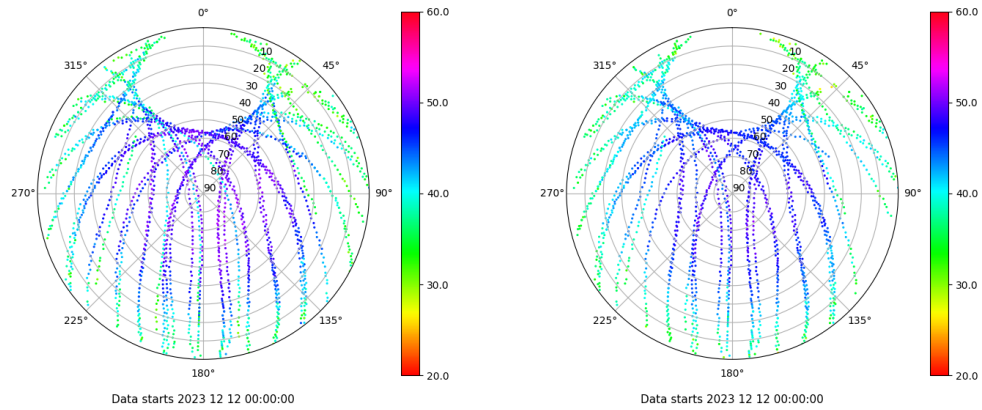
Skyplot for station MAL1. Signal to Noise S1C Data file MAL100ESP_R_2023346.xtr Skyplot for station MAL1. Signal to Noise S2P Data file MAL100ESP_R_2023346.xtr
