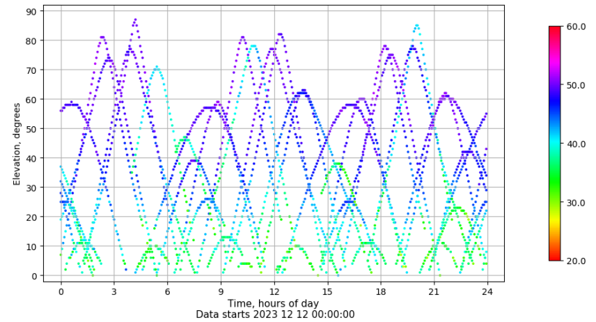
Time-elevation plot for station MAL1. Signal to Noise S1C Data file MAL100ESP_R_2023346.xtr
