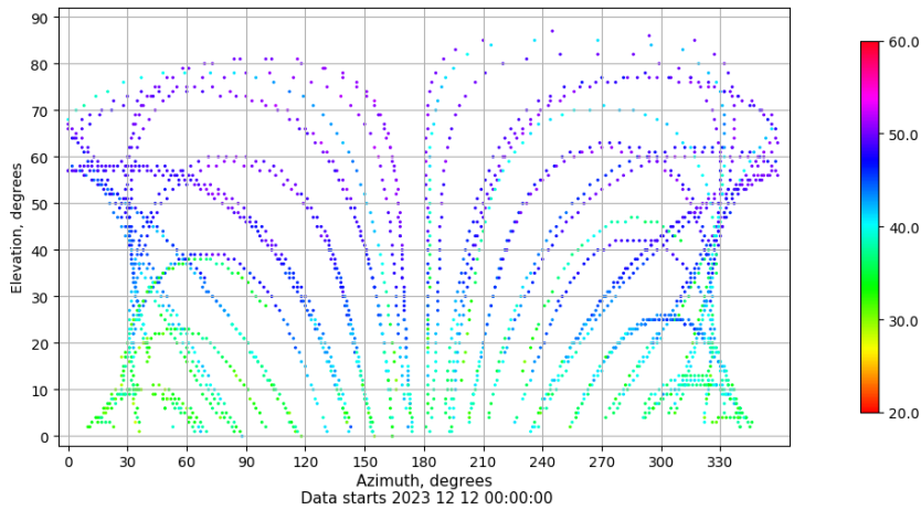
Azimuth-elevation plot for station MAL1. Signal to Noise S1C Data file MAL100ESP_R_2023346.xtr
