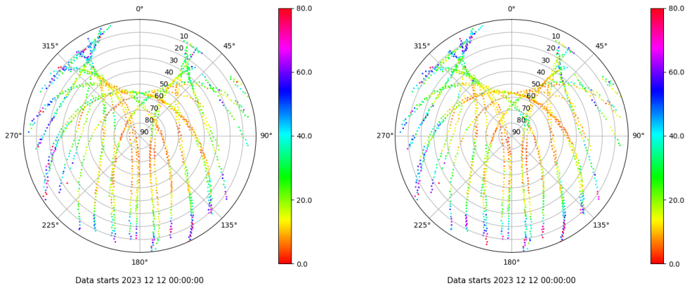
Skyplot for station MAL1. Parameter M1C Data file MAL100ESP_R_2023346.xtr Skyplot for station MAL1. Parameter M2P Data file MAL100ESP_R_2023346.xtr
