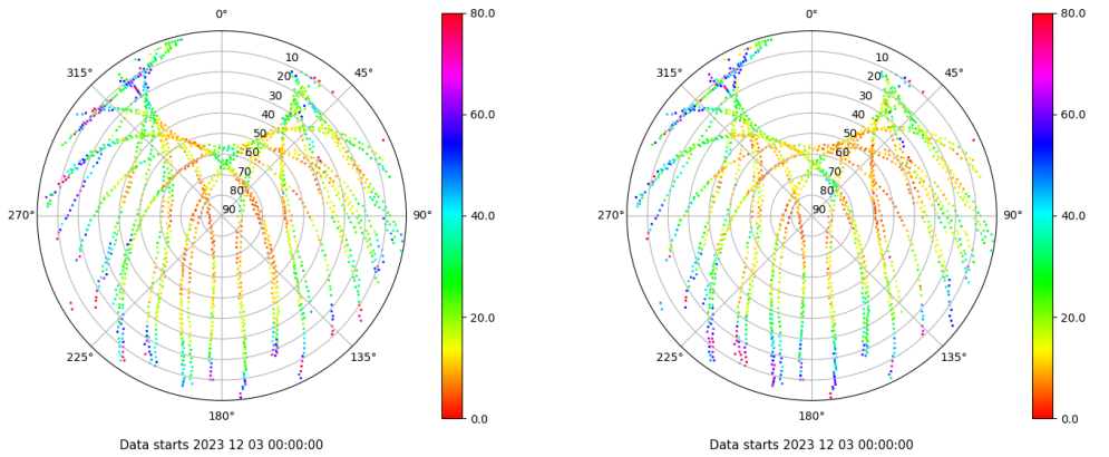
Skyplot for station MAL1. Parameter M1C Data file MAL100ESP_R_2023337.xtr Skyplot for station MAL1. Parameter M2P Data file MAL100ESP_R_2023337.xtr
