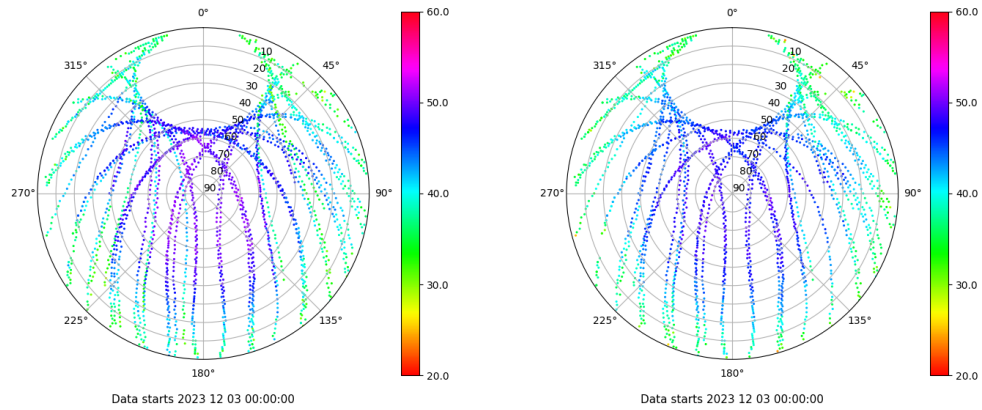
Skyplot for station MAL1. Signal to Noise S1C Data file MAL100ESP_R_2023337.xtr Skyplot for station MAL1. Signal to Noise S2P Data file MAL100ESP_R_2023337.xtr
