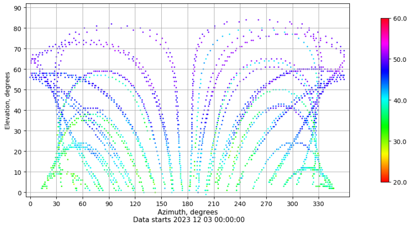
Azimuth-elevation plot for station MAL1. Signal to Noise S1C Data file MAL100ESP_R_2023337.xtr
