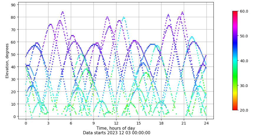
Time-elevation plot for station MAL1. Signal to Noise S1C Data file MAL100ESP_R_2023337.xtr
