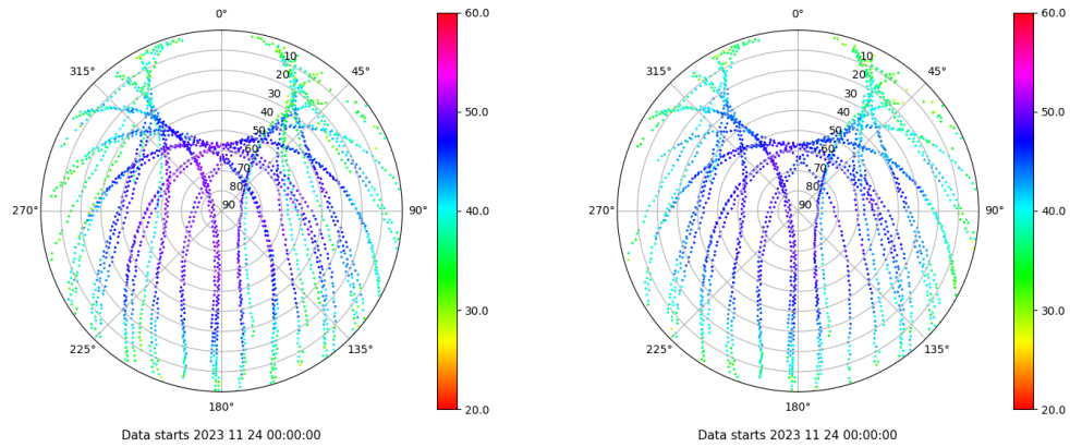
Skyplot for station MAL1. Signal to Noise S1C Data file MAL100ESP_R_2023328.xtr Skyplot for station MAL1. Signal to Noise S2P Data file MAL100ESP_R_2023328.xtr
