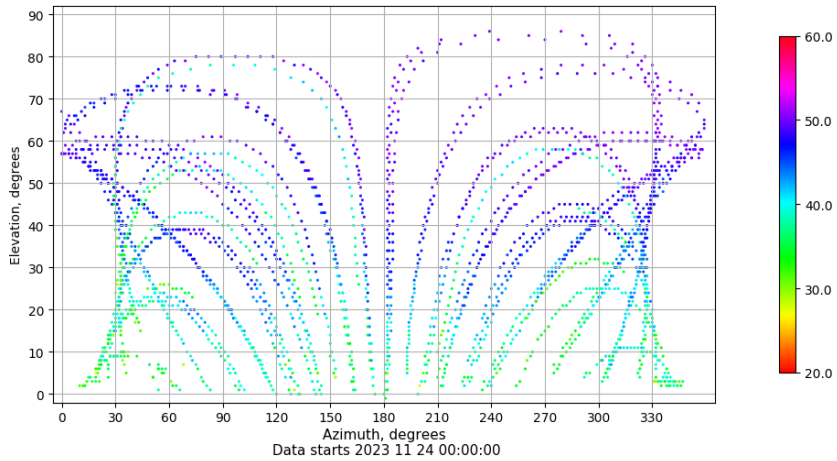
Azimuth-elevation plot for station MAL1. Signal to Noise S1C Data file MAL100ESP_R_2023328.xtr
