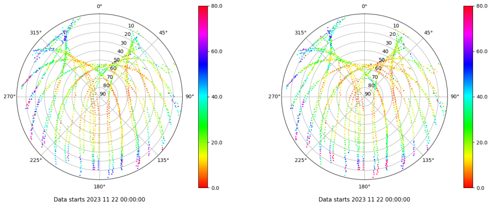
Skyplot for station MAL1. Parameter M1C Data file MAL100ESP_R_2023326.xtr Skyplot for station MAL1. Parameter M2P Data file MAL100ESP_R_2023326.xtr
