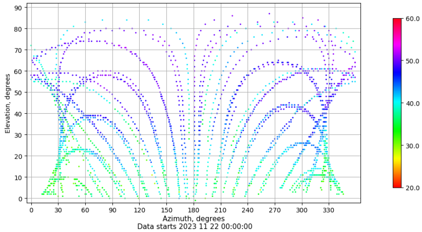
Azimuth-elevation plot for station MAL1. Signal to Noise S1C Data file MAL100ESP_R_2023326.xtr
