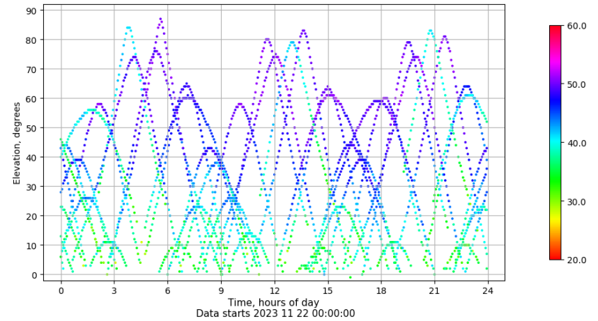
Time-elevation plot for station MAL1. Signal to Noise S1C Data file MAL100ESP_R_2023326.xtr
