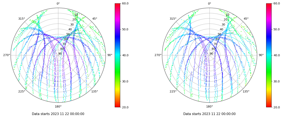
Skyplot for station MAL1. Signal to Noise S1C Data file MAL100ESP_R_2023326.xtr Skyplot for station MAL1. Signal to Noise S2P Data file MAL100ESP_R_2023326.xtr
