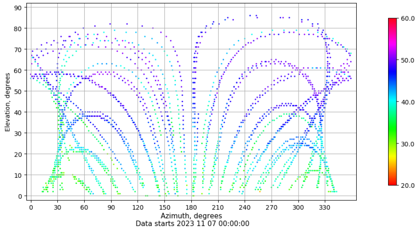
Azimuth-elevation plot for station MAL1. Signal to Noise S1C Data file MAL100ESP_R_2023311.xtr
