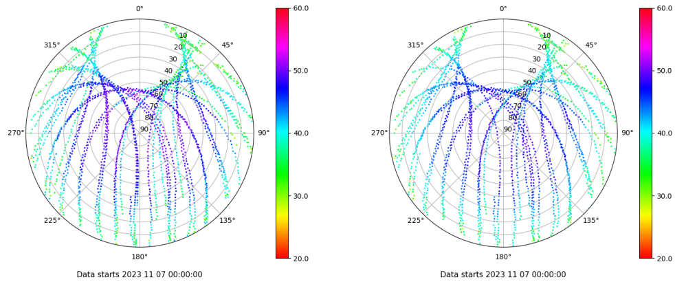
Skyplot for station MAL1. Signal to Noise S1C Data file MAL100ESP_R_2023311.xtr Skyplot for station MAL1. Signal to Noise S2P Data file MAL100ESP_R_2023311.xtr
