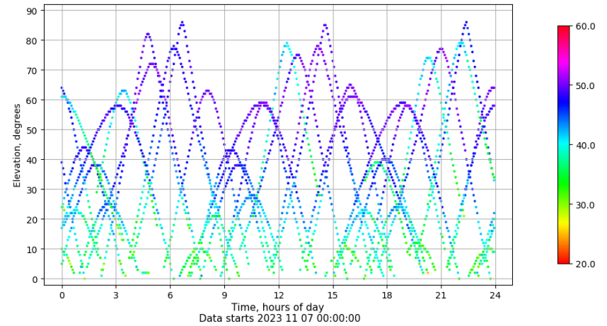
Time-elevation plot for station MAL1. Signal to Noise S1C Data file MAL100ESP_R_2023311.xtr
