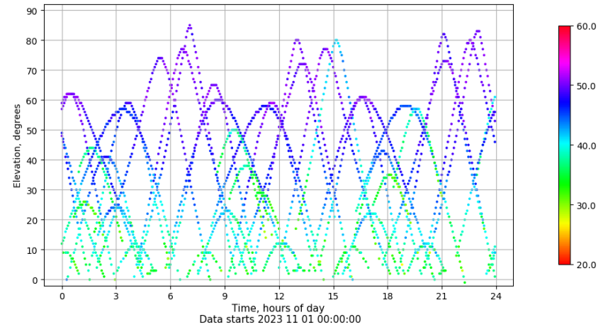
Time-elevation plot for station MAL1. Signal to Noise S1C Data file MAL100ESP_R_2023305.xtr
