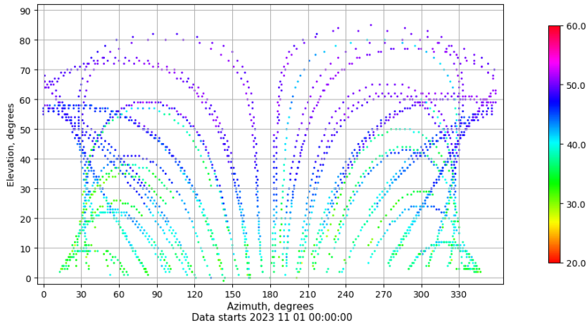
Azimuth-elevation plot for station MAL1. Signal to Noise S1C Data file MAL100ESP_R_2023305.xtr
