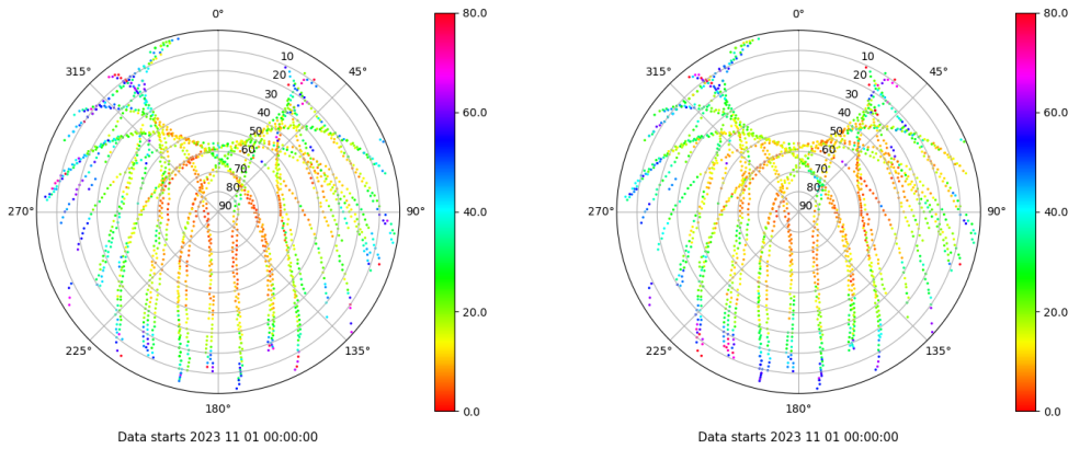
Skyplot for station MAL1. Parameter M1C Data file MAL100ESP_R_2023305.xtr Skyplot for station MAL1. Parameter M2P Data file MAL100ESP_R_2023305.xtr
