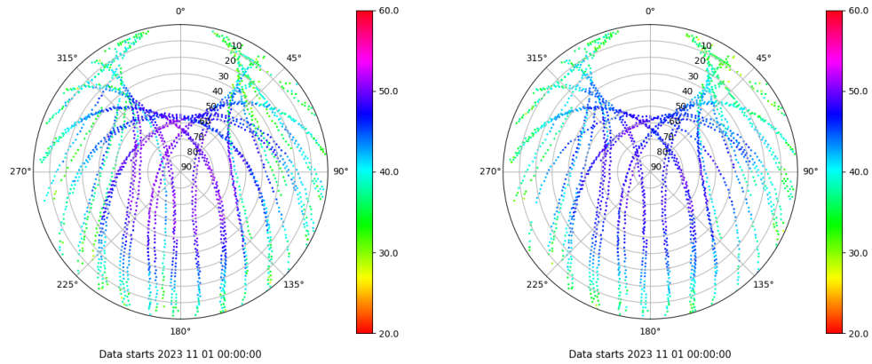
Skyplot for station MAL1. Signal to Noise S1C Data file MAL100ESP_R_2023305.xtr Skyplot for station MAL1. Signal to Noise S2P Data file MAL100ESP_R_2023305.xtr
