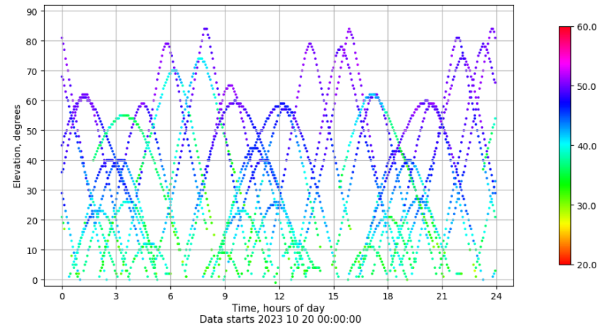
Time-elevation plot for station MAL1. Signal to Noise S1C Data file MAL100ESP_R_2023293.xtr
