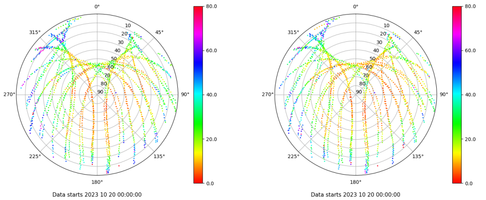
Skyplot for station MAL1. Parameter M1C Data file MAL100ESP_R_2023293.xtr Skyplot for station MAL1. Parameter M2P Data file MAL100ESP_R_2023293.xtr
