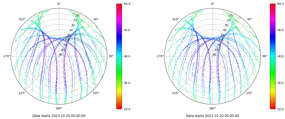
Skyplot for station MAL1. Signal to Noise S1C Data file MAL100ESP_R_2023293.xtr Skyplot for station MAL1. Signal to Noise S2P Data file MAL100ESP_R_2023293.xtr
