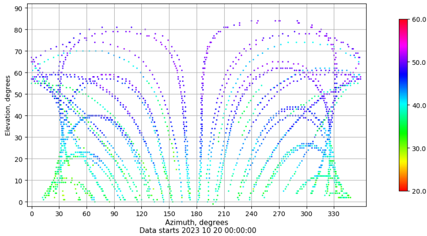
Azimuth-elevation plot for station MAL1. Signal to Noise S1C Data file MAL100ESP_R_2023293.xtr
