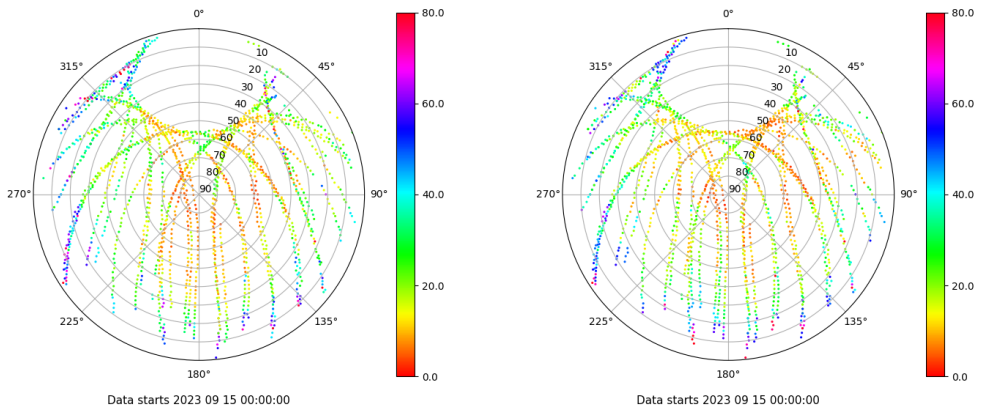
Skyplot for station MAL1. Parameter M1C Data file MAL100ESP_R_2023258.xtr Skyplot for station MAL1. Parameter M2P Data file MAL100ESP_R_2023258.xtr
