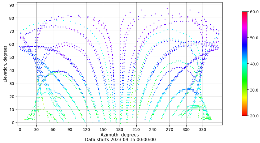
Azimuth-elevation plot for station MAL1. Signal to Noise S1C Data file MAL100ESP_R_2023258.xtr
