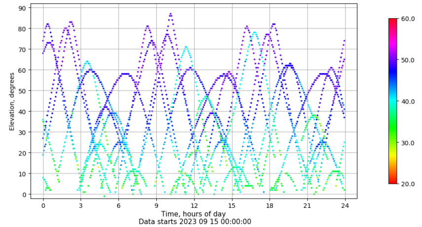
Time-elevation plot for station MAL1. Signal to Noise S1C Data file MAL100ESP_R_2023258.xtr
