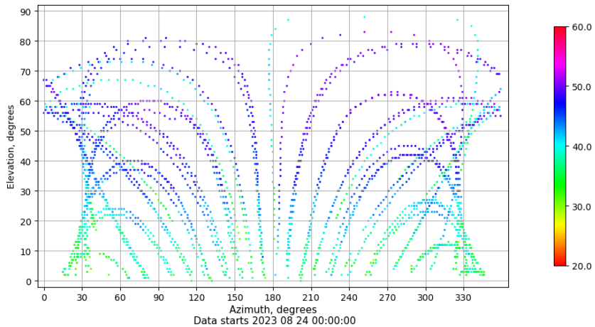
Azimuth-elevation plot for station MAL1. Signal to Noise S1C Data file MAL100ESP_R_2023236.xtr
