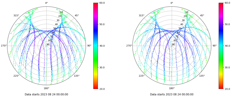
Skyplot for station MAL1. Signal to Noise S1C Data file MAL100ESP_R_2023236.xtr Skyplot for station MAL1. Signal to Noise S2P Data file MAL100ESP_R_2023236.xtr
