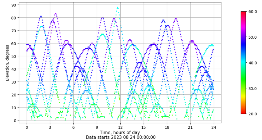
Time-elevation plot for station MAL1. Signal to Noise S1C Data file MAL100ESP_R_2023236.xtr
