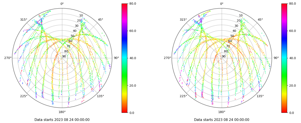
Skyplot for station MAL1. Parameter M1C Data file MAL100ESP_R_2023236.xtr Skyplot for station MAL1. Parameter M2P Data file MAL100ESP_R_2023236.xtr
