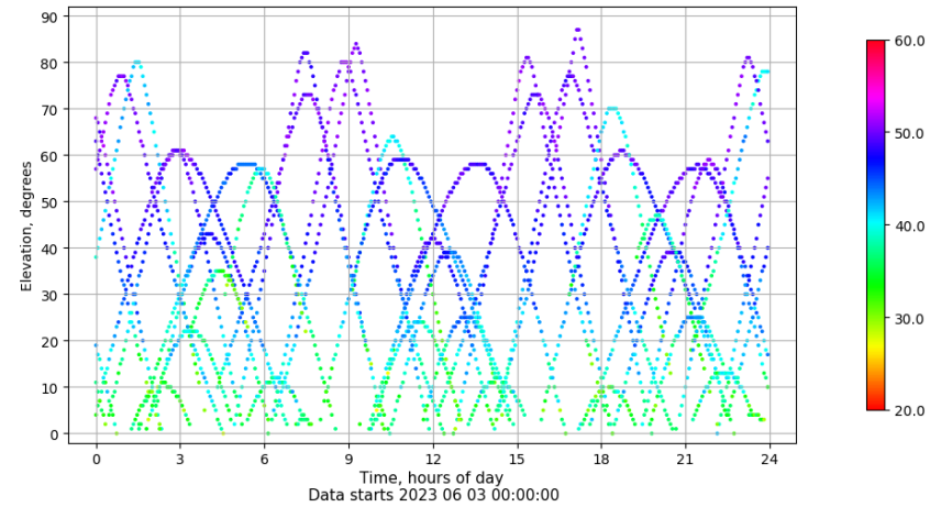
Time-elevation plot for station MAL1. Signal to Noise S1C Data file MAL100ESP_R_2023154.xtr
