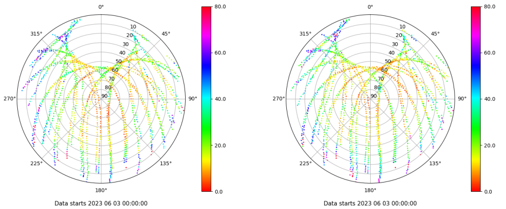
Skyplot for station MAL1. Parameter M1C Data file MAL100ESP_R_2023154.xtr Skyplot for station MAL1. Parameter M2P Data file MAL100ESP_R_2023154.xtr
