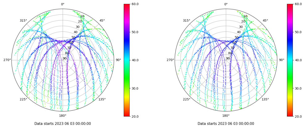
Skyplot for station MAL1. Signal to Noise S1C Data file MAL100ESP_R_2023154.xtr Skyplot for station MAL1. Signal to Noise S2P Data file MAL100ESP_R_2023154.xtr
