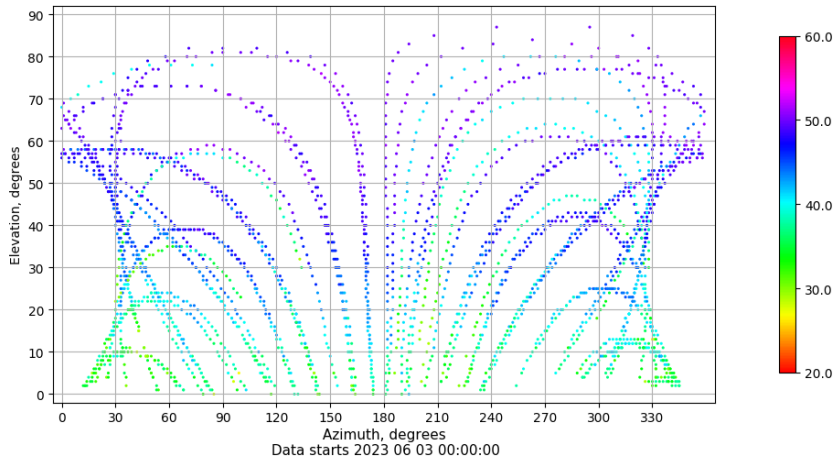
Azimuth-elevation plot for station MAL1. Signal to Noise S1C Data file MAL100ESP_R_2023154.xtr
