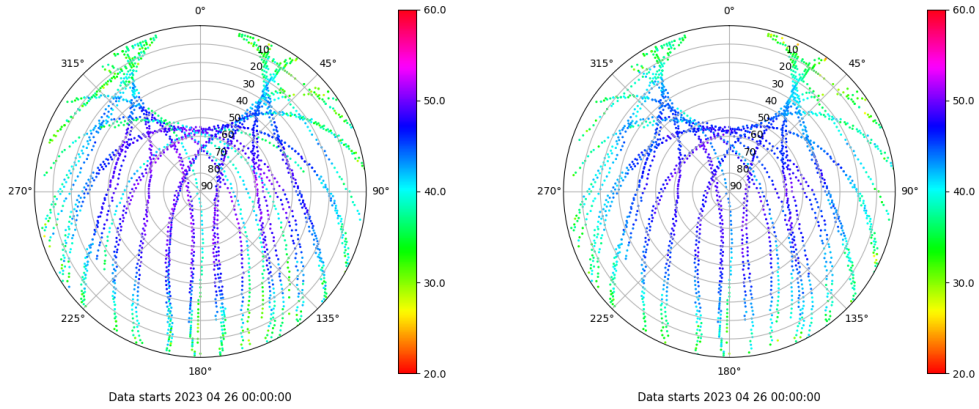
Skyplot for station MAL1. Signal to Noise S1C Data file MAL100ESP_R_2023116.xtr Skyplot for station MAL1. Signal to Noise S2P Data file MAL100ESP_R_2023116.xtr
