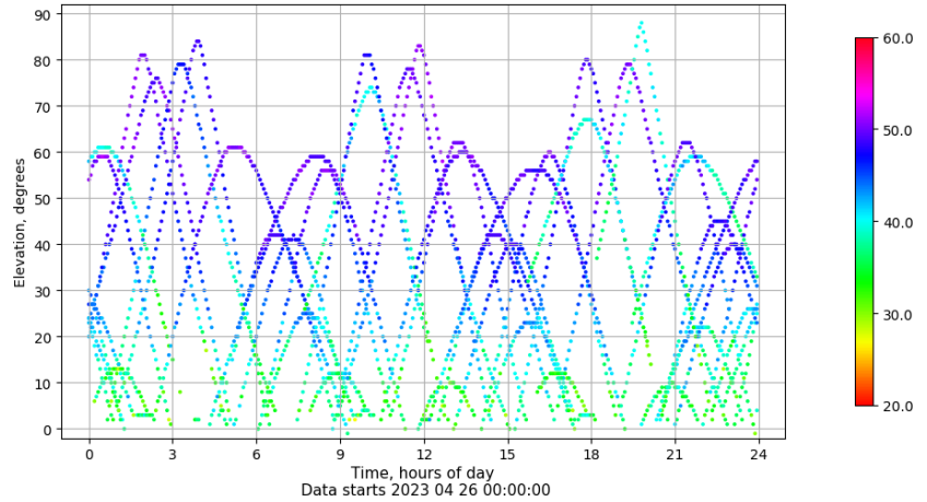
Time-elevation plot for station MAL1. Signal to Noise S1C Data file MAL100ESP_R_2023116.xtr
