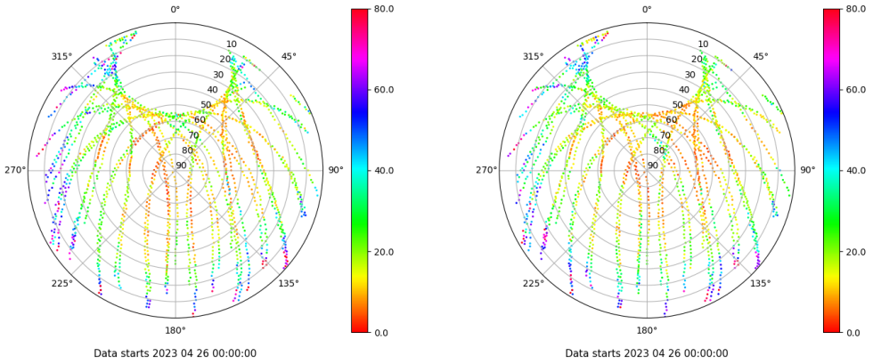
Skyplot for station MAL1. Parameter M1C Data file MAL100ESP_R_2023116.xtr Skyplot for station MAL1. Parameter M2P Data file MAL100ESP_R_2023116.xtr
