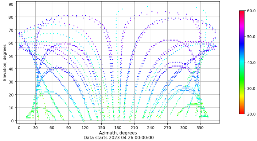
Azimuth-elevation plot for station MAL1. Signal to Noise S1C Data file MAL100ESP_R_2023116.xtr
