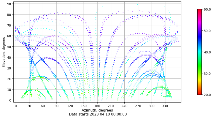
Azimuth-elevation plot for station MAL1. Signal to Noise S1C Data file MAL100ESP_R_2023100.xtr
