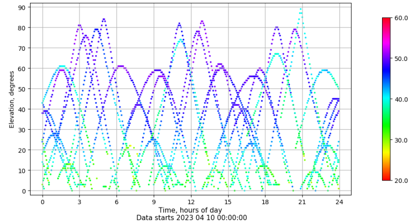
Time-elevation plot for station MAL1. Signal to Noise S1C Data file MAL100ESP_R_2023100.xtr
