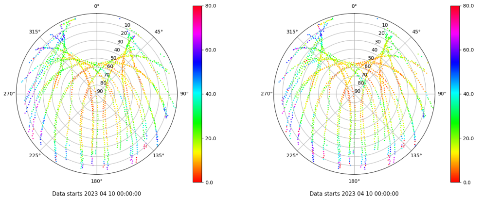
Skyplot for station MAL1. Parameter M1C Data file MAL100ESP_R_2023100.xtr Skyplot for station MAL1. Parameter M2P Data file MAL100ESP_R_2023100.xtr
