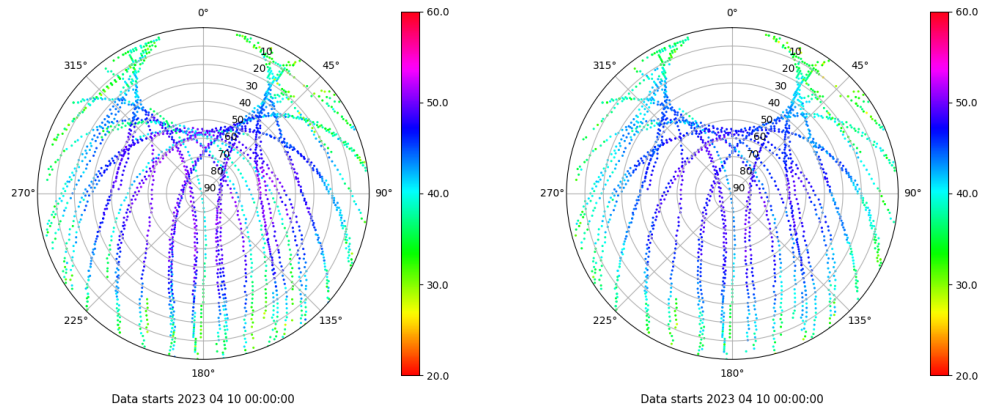
Skyplot for station MAL1. Signal to Noise S1C Data file MAL100ESP_R_2023100.xtr Skyplot for station MAL1. Signal to Noise S2P Data file MAL100ESP_R_2023100.xtr
