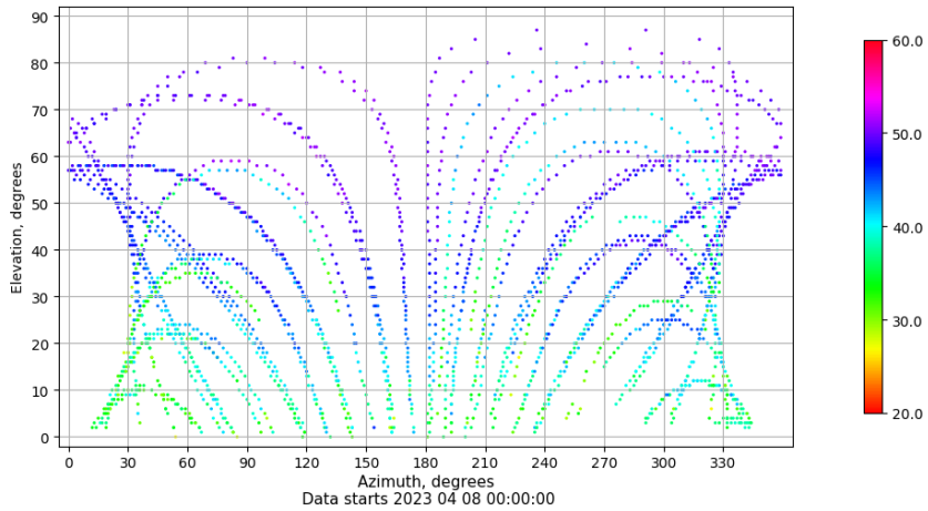
Azimuth-elevation plot for station MAL1. Signal to Noise S1C Data file MAL100ESP_R_2023098.xtr
