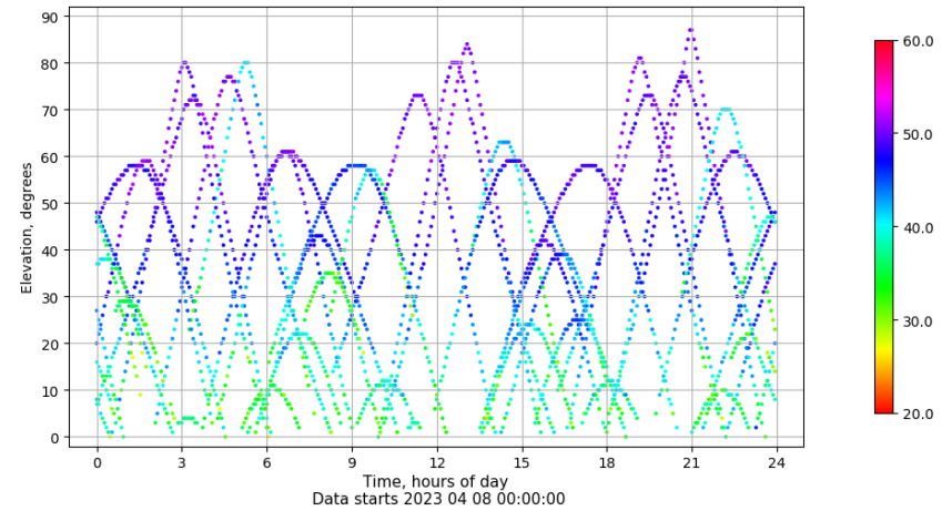
Time-elevation plot for station MAL1. Signal to Noise S1C Data file MAL100ESP_R_2023098.xtr
