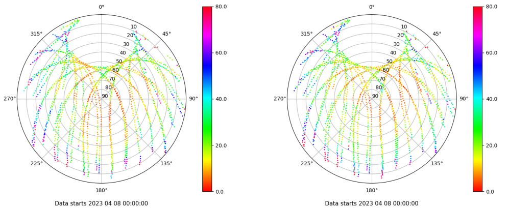
Skyplot for station MAL1. Parameter M1C Data file MAL100ESP_R_2023098.xtr Skyplot for station MAL1. Parameter M2P Data file MAL100ESP_R_2023098.xtr
