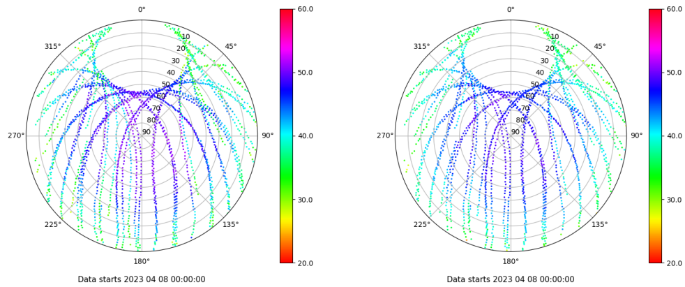
Skyplot for station MAL1. Signal to Noise S1C Data file MAL100ESP_R_2023098.xtr Skyplot for station MAL1. Signal to Noise S2P Data file MAL100ESP_R_2023098.xtr
