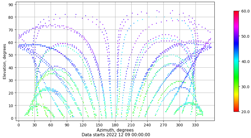
Azimuth-elevation plot for station MAL1. Signal to Noise S1C Data file MAL100ESP_R_2022343.xtr
