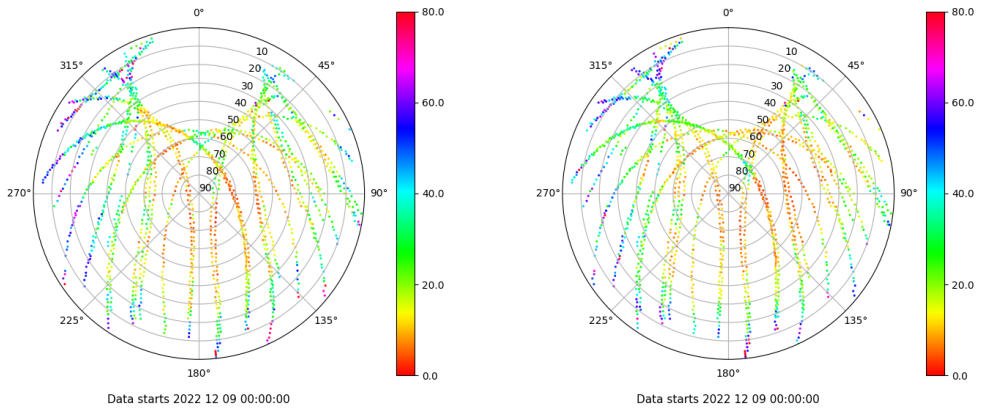
Skyplot for station MAL1. Parameter M1C Data file MAL100ESP_R_2022343.xtr Skyplot for station MAL1. Parameter M2P Data file MAL100ESP_R_2022343.xtr
