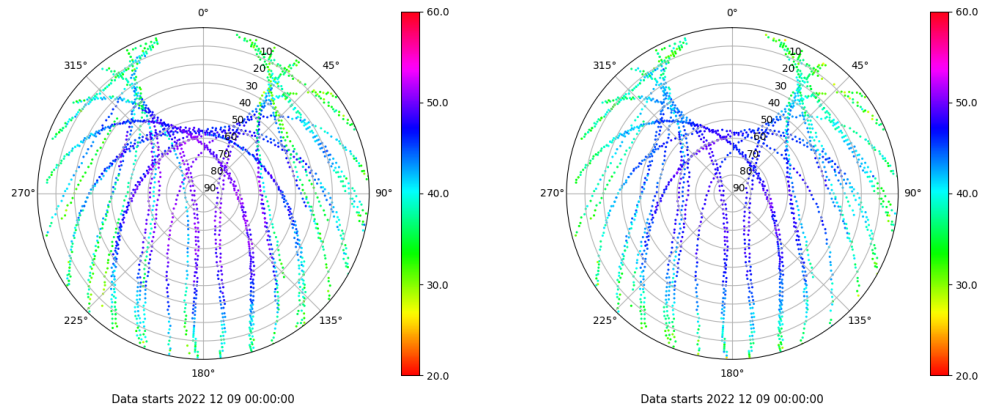
Skyplot for station MAL1. Signal to Noise S1C Data file MAL100ESP_R_2022343.xtr Skyplot for station MAL1. Signal to Noise S2P Data file MAL100ESP_R_2022343.xtr
