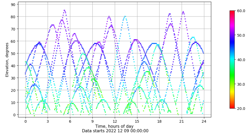
Time-elevation plot for station MAL1. Signal to Noise S1C Data file MAL100ESP_R_2022343.xtr
