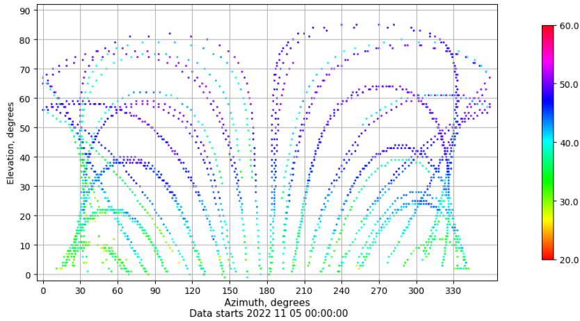
Azimuth-elevation plot for station MAL1. Signal to Noise S1C Data file MAL100ESP_R_2022309.xtr
