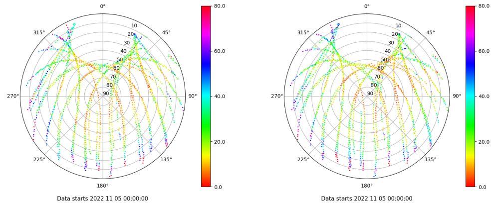
Skyplot for station MAL1. Parameter M1C Data file MAL100ESP_R_2022309.xtr Skyplot for station MAL1. Parameter M2P Data file MAL100ESP_R_2022309.xtr
