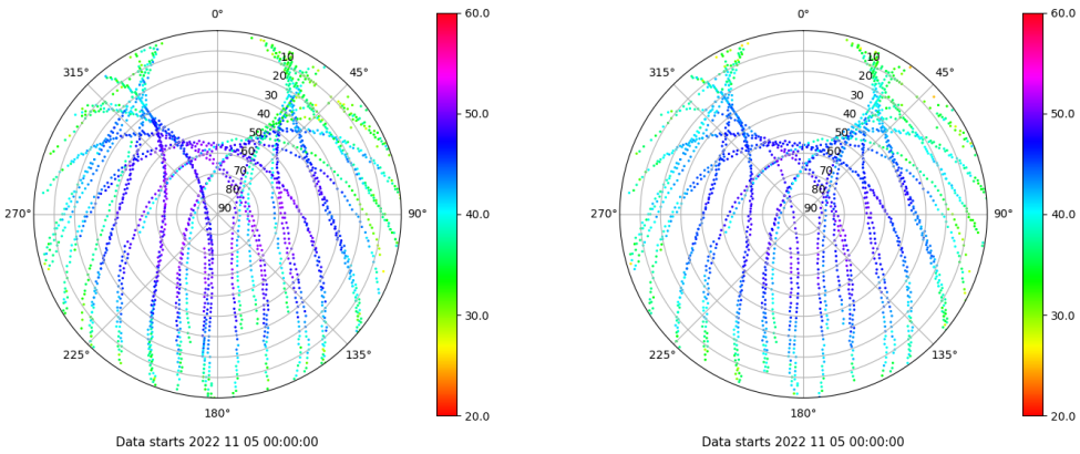
Skyplot for station MAL1. Signal to Noise S1C Data file MAL100ESP_R_2022309.xtr Skyplot for station MAL1. Signal to Noise S2P Data file MAL100ESP_R_2022309.xtr
