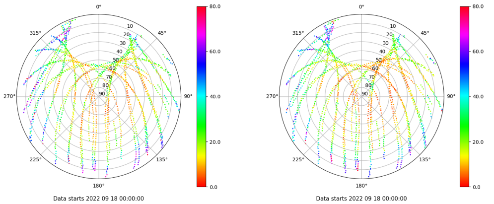
Skyplot for station MAL1. Parameter M1C Data file MAL100ESP_R_2022261.xtr Skyplot for station MAL1. Parameter M2P Data file MAL100ESP_R_2022261.xtr
