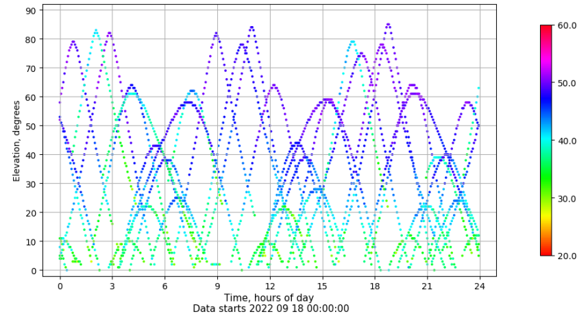
Time-elevation plot for station MAL1. Signal to Noise S1C Data file MAL100ESP_R_2022261.xtr
