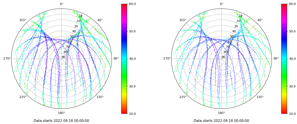
Skyplot for station MAL1. Signal to Noise S1C Data file MAL100ESP_R_2022261.xtr Skyplot for station MAL1. Signal to Noise S2P Data file MAL100ESP_R_2022261.xtr
