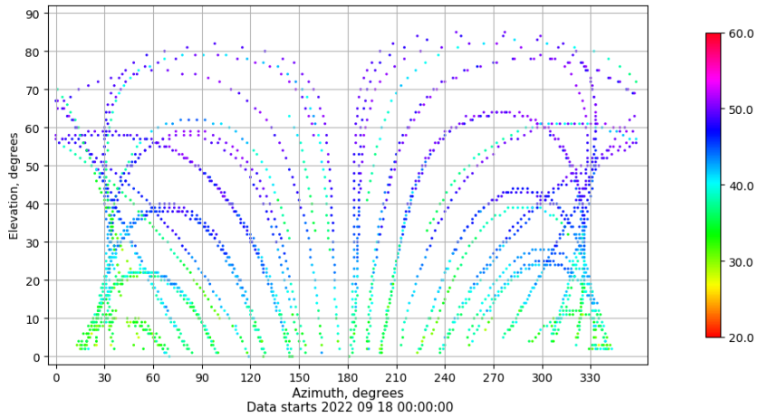
Azimuth-elevation plot for station MAL1. Signal to Noise S1C Data file MAL100ESP_R_2022261.xtr
