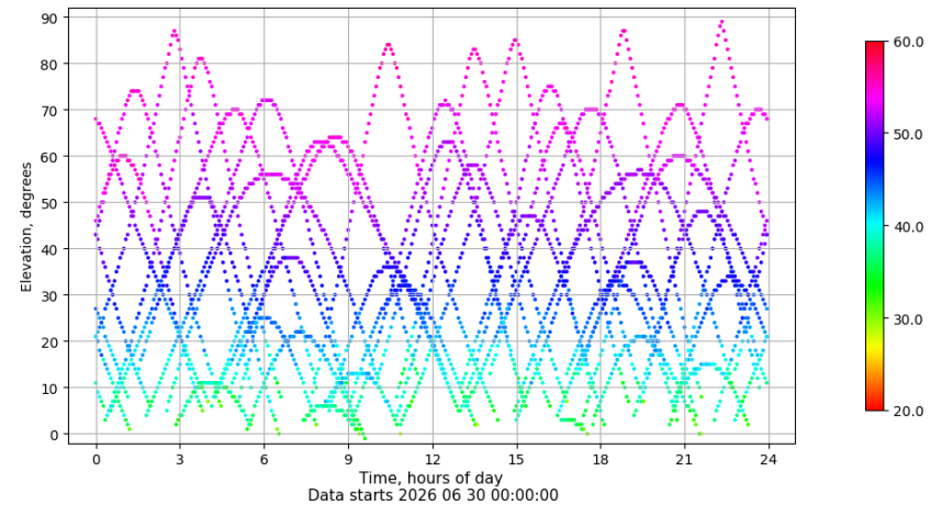
Time-elevation plot for station LPAL. Signal to Noise S1C Data file LPAL00ESP_R_2026181.xtr
