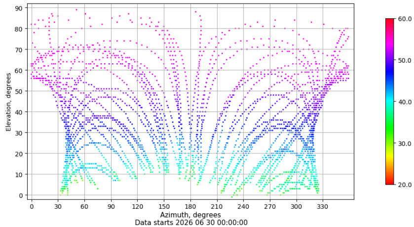
Azimuth-elevation plot for station LPAL. Signal to Noise S1C Data file LPAL00ESP_R_2026181.xtr
