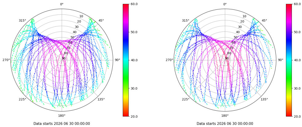
Skyplot for station LPAL. Signal to Noise S1C Data file LPAL00ESP_R_2026181.xtr Skyplot for station LPAL. Signal to Noise S2S Data file LPAL00ESP_R_2026181.xtr
