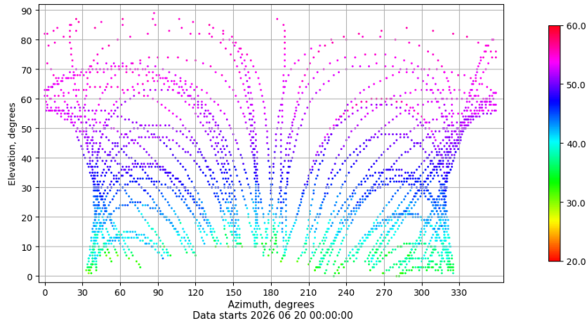
Azimuth-elevation plot for station LPAL. Signal to Noise S1C Data file LPAL00ESP_R_2026171.xtr
