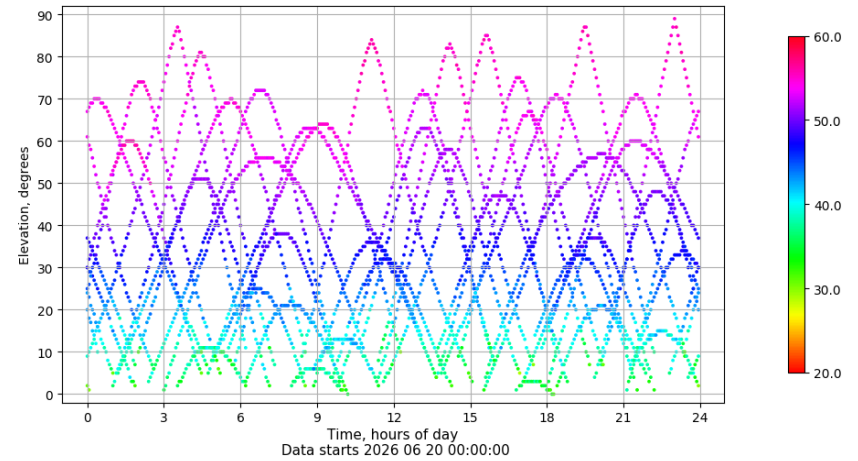
Time-elevation plot for station LPAL. Signal to Noise S1C Data file LPAL00ESP_R_2026171.xtr
