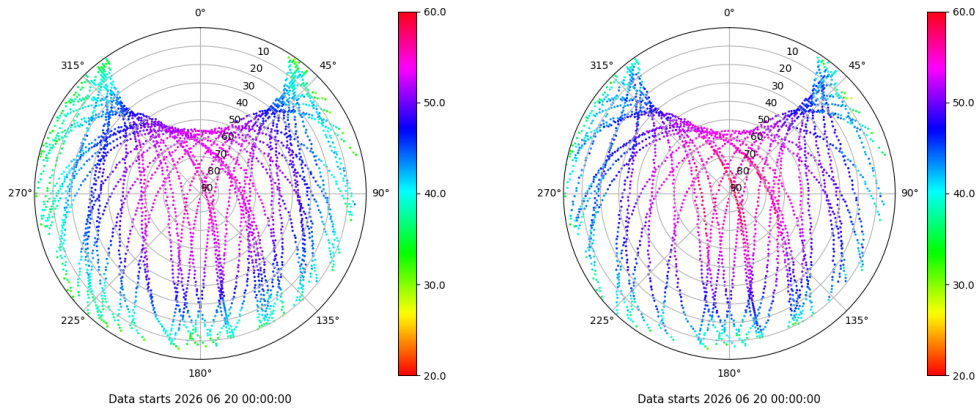
Skyplot for station LPAL. Signal to Noise S1C Data file LPAL00ESP_R_2026171.xtr Skyplot for station LPAL. Signal to Noise S2S Data file LPAL00ESP_R_2026171.xtr
