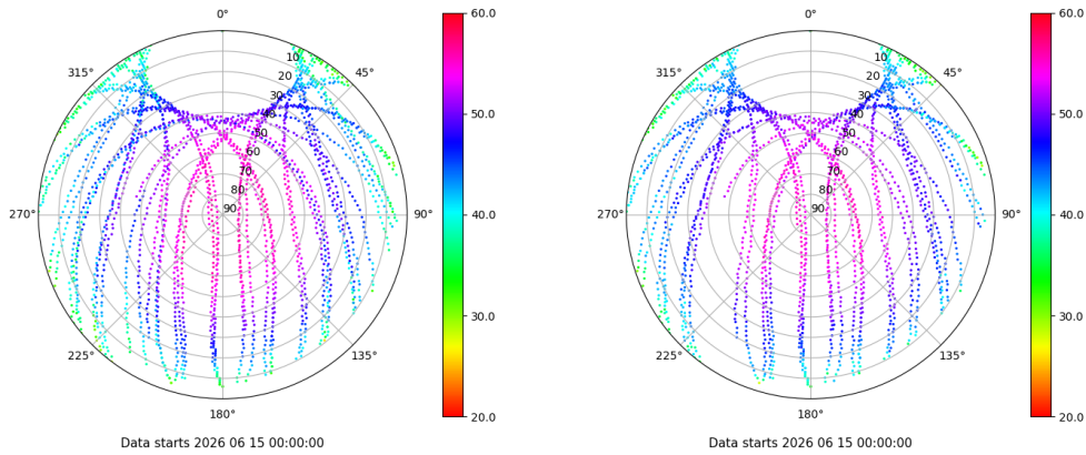
Skyplot for station LPAL. Signal to Noise S1C Data file LPAL00ESP_R_2026166.xtr Skyplot for station LPAL. Signal to Noise S2C Data file LPAL00ESP_R_2026166.xtr
