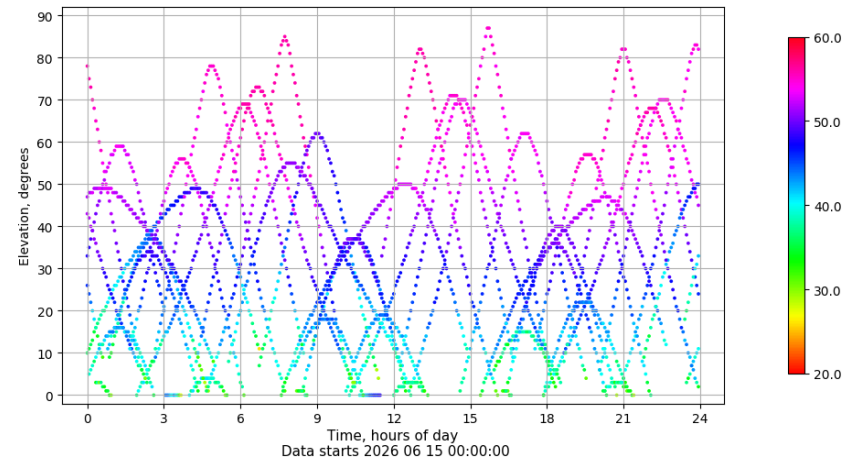
Time-elevation plot for station LPAL. Signal to Noise S1C Data file LPAL00ESP_R_2026166.xtr
