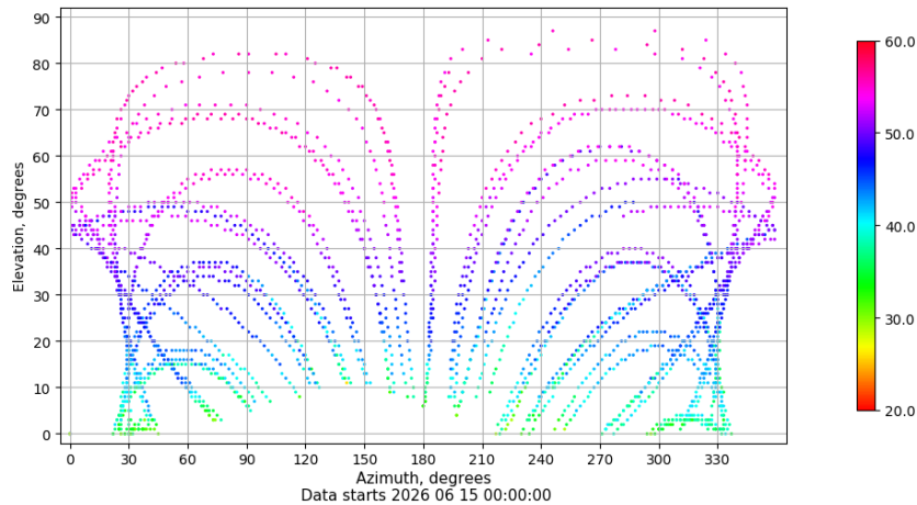
Azimuth-elevation plot for station LPAL. Signal to Noise S1C Data file LPAL00ESP_R_2026166.xtr
