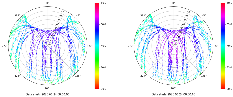
Skyplot for station LP01. Signal to Noise S1X Data file LP0100ESP_R_2026175.xtr Skyplot for station LP01. Signal to Noise S5X Data file LP0100ESP_R_2026175.xtr
