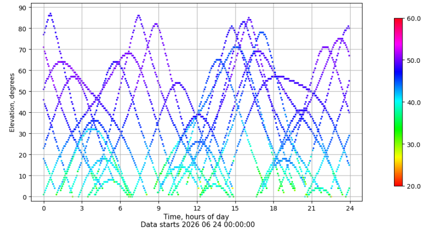
Time-elevation plot for station LP01. Signal to Noise S1X Data file LP0100ESP_R_2026175.xtr
