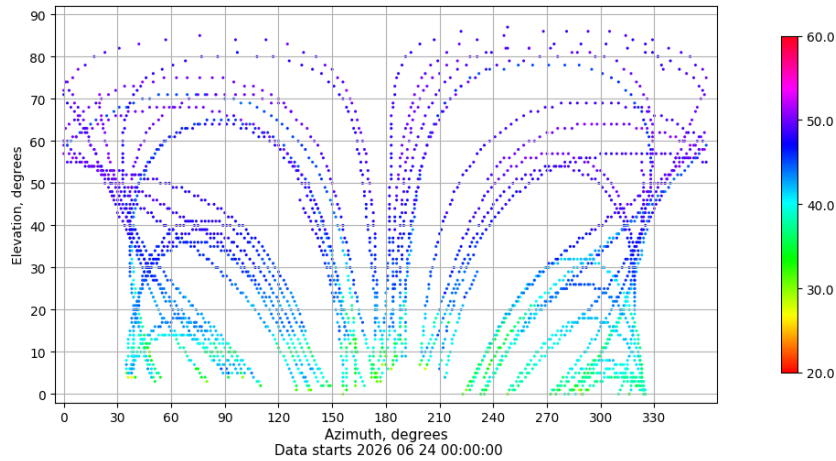
Azimuth-elevation plot for station LP01. Signal to Noise S1X Data file LP0100ESP_R_2026175.xtr
