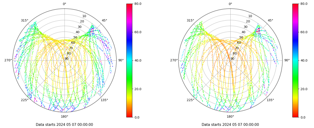
Skyplot for station LALA. Parameter M1C Data file LALA00ESP_R_2024128.xtr Skyplot for station LALA. Parameter M2X Data file LALA00ESP_R_2024128.xtr
