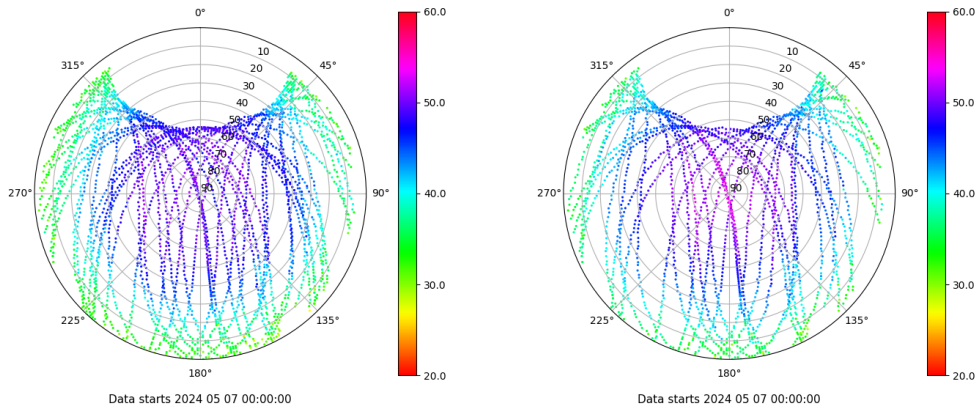
Skyplot for station LALA. Signal to Noise S1C Data file LALA00ESP_R_2024128.xtr Skyplot for station LALA. Signal to Noise S2X Data file LALA00ESP_R_2024128.xtr
