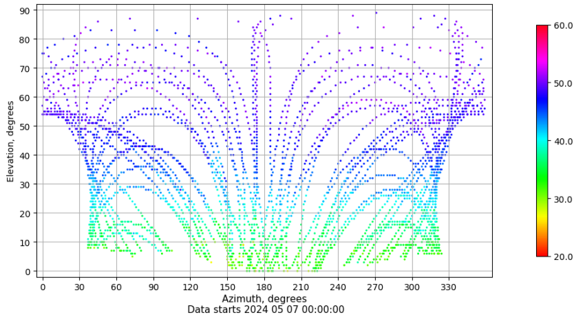
Azimuth-elevation plot for station LALA. Signal to Noise S1C Data file LALA00ESP_R_2024128.xtr
