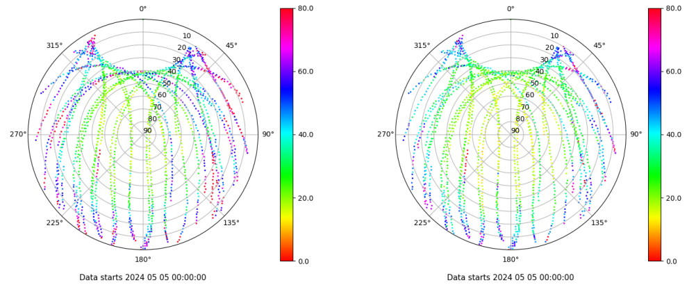
Skyplot for station LALA. Parameter M1C Data file LALA00ESP_R_2024126.xtr Skyplot for station LALA. Parameter M2C Data file LALA00ESP_R_2024126.xtr
