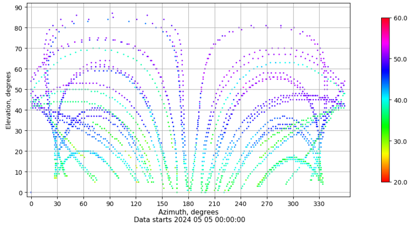
Azimuth-elevation plot for station LALA. Signal to Noise S1C Data file LALA00ESP_R_2024126.xtr
