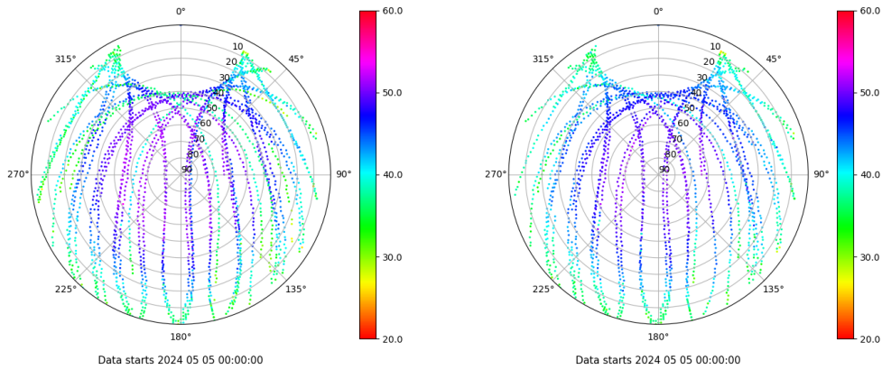
Skyplot for station LALA. Signal to Noise S1C Data file LALA00ESP_R_2024126.xtr Skyplot for station LALA. Signal to Noise S2C Data file LALA00ESP_R_2024126.xtr
