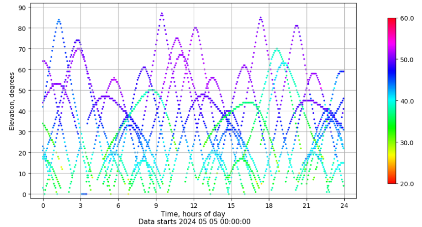
Time-elevation plot for station LALA. Signal to Noise S1C Data file LALA00ESP_R_2024126.xtr
