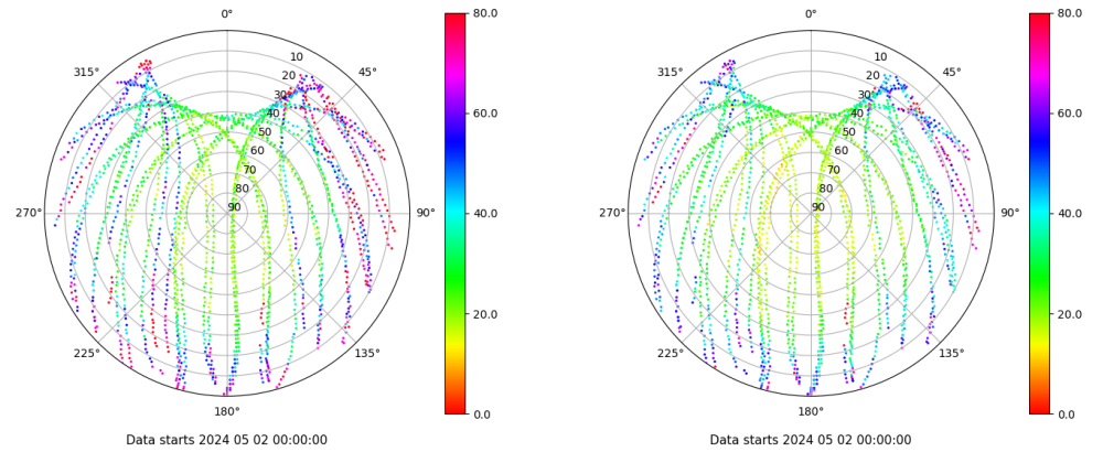
Skyplot for station LALA. Parameter M1C Data file LALA00ESP_R_2024123.xtr Skyplot for station LALA. Parameter M2C Data file LALA00ESP_R_2024123.xtr
