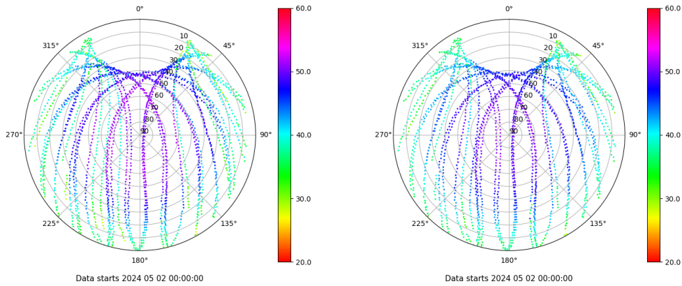
Skyplot for station LALA. Signal to Noise S1C Data file LALA00ESP_R_2024123.xtr Skyplot for station LALA. Signal to Noise S2C Data file LALA00ESP_R_2024123.xtr
