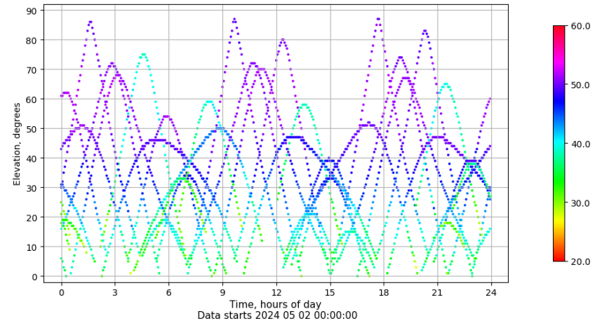
Time-elevation plot for station LALA. Signal to Noise S1C Data file LALA00ESP_R_2024123.xtr
