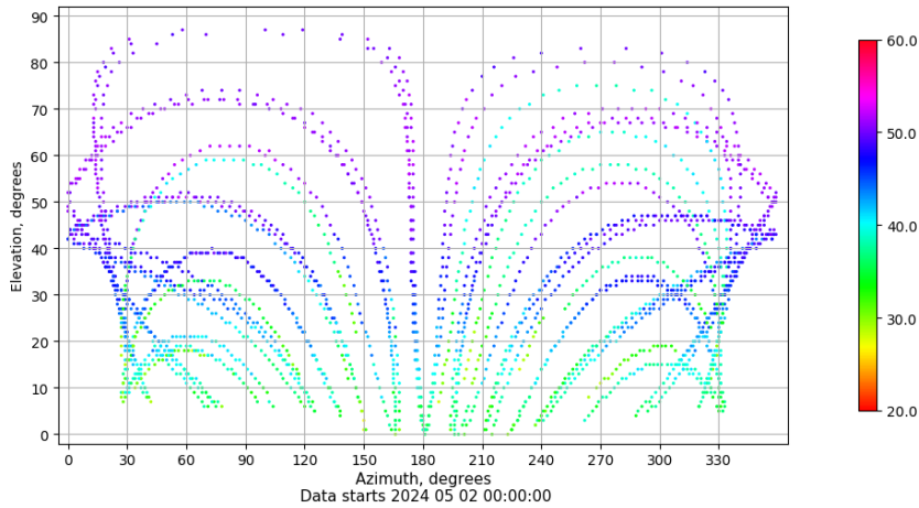
Azimuth-elevation plot for station LALA. Signal to Noise S1C Data file LALA00ESP_R_2024123.xtr
