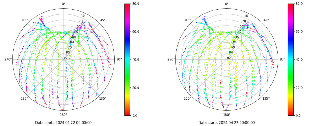
Skyplot for station LALA. Parameter M1C Data file LALA00ESP_R_2024113.xtr Skyplot for station LALA. Parameter M2C Data file LALA00ESP_R_2024113.xtr
