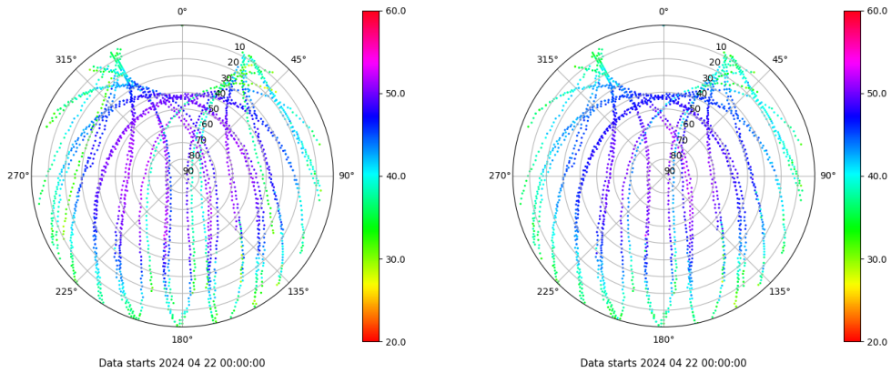
Skyplot for station LALA. Signal to Noise S1C Data file LALA00ESP_R_2024113.xtr Skyplot for station LALA. Signal to Noise S2C Data file LALA00ESP_R_2024113.xtr
