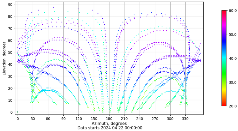
Azimuth-elevation plot for station LALA. Signal to Noise S1C Data file LALA00ESP_R_2024113.xtr
