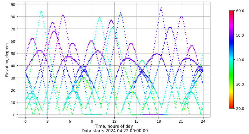
Time-elevation plot for station LALA. Signal to Noise S1C Data file LALA00ESP_R_2024113.xtr
