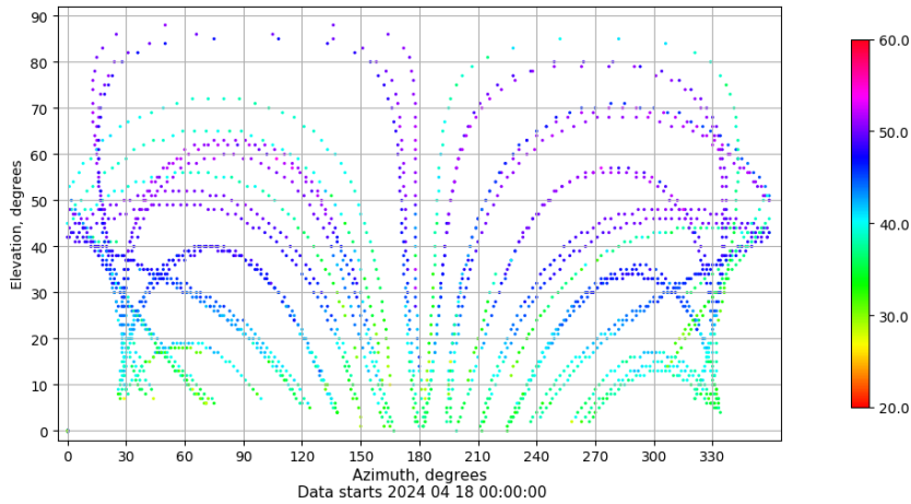
Azimuth-elevation plot for station LALA. Signal to Noise S1C Data file LALA00ESP_R_2024109.xtr
