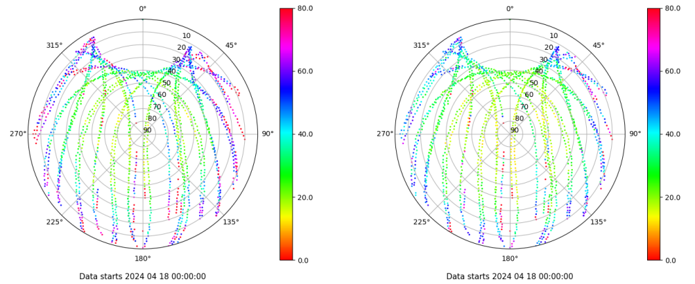
Skyplot for station LALA. Parameter M1C Data file LALA00ESP_R_2024109.xtr Skyplot for station LALA. Parameter M2C Data file LALA00ESP_R_2024109.xtr
