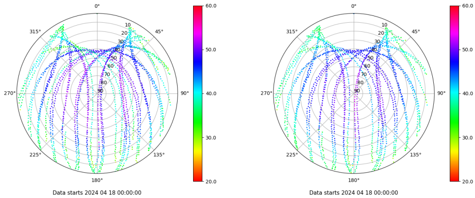
Skyplot for station LALA. Signal to Noise S1C Data file LALA00ESP_R_2024109.xtr Skyplot for station LALA. Signal to Noise S2C Data file LALA00ESP_R_2024109.xtr
