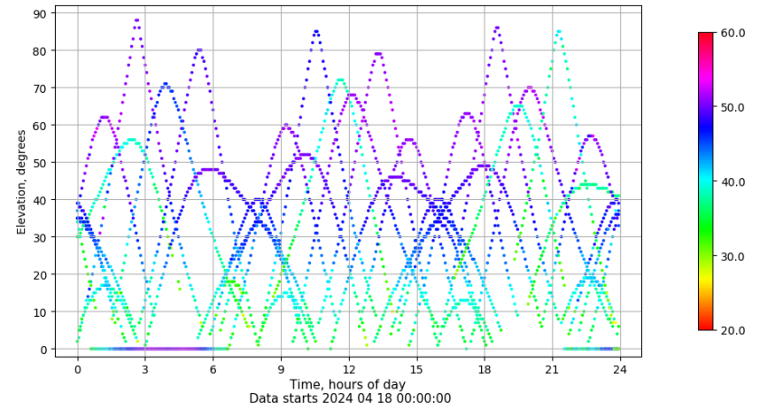
Time-elevation plot for station LALA. Signal to Noise S1C Data file LALA00ESP_R_2024109.xtr
