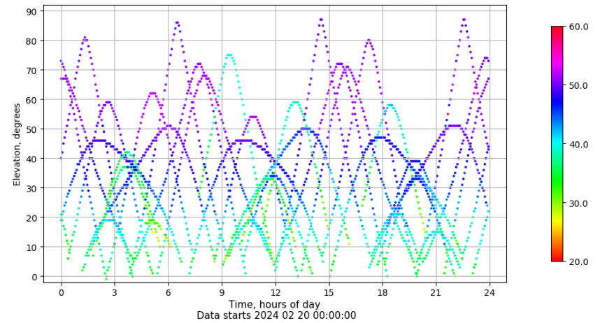
Time-elevation plot for station LALA. Signal to Noise S1C Data file LALA00ESP_R_2024051.xtr
