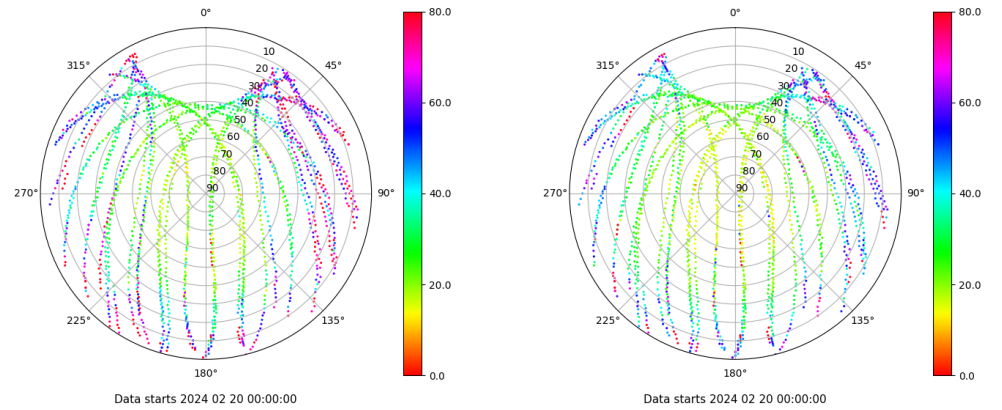
Skyplot for station LALA. Parameter M1C Data file LALA00ESP_R_2024051.xtr Skyplot for station LALA. Parameter M2C Data file LALA00ESP_R_2024051.xtr
