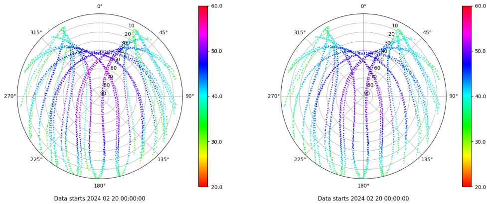
Skyplot for station LALA. Signal to Noise S1C Data file LALA00ESP_R_2024051.xtr Skyplot for station LALA. Signal to Noise S2C Data file LALA00ESP_R_2024051.xtr
