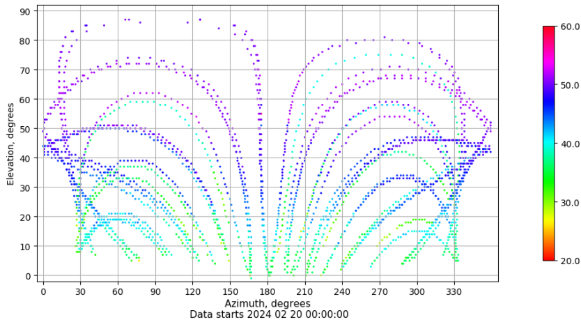
Azimuth-elevation plot for station LALA. Signal to Noise S1C Data file LALA00ESP_R_2024051.xtr
