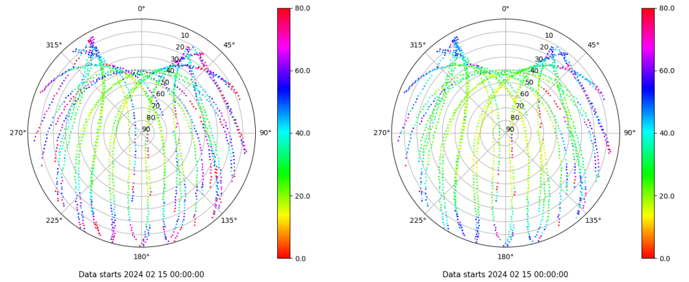
Skyplot for station LALA. Parameter M1C Data file LALA00ESP_R_2024046.xtr Skyplot for station LALA. Parameter M2C Data file LALA00ESP_R_2024046.xtr
