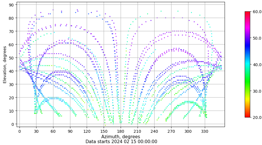
Azimuth-elevation plot for station LALA. Signal to Noise S1C Data file LALA00ESP_R_2024046.xtr
