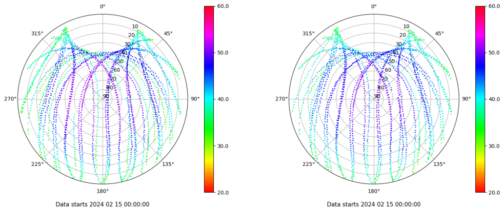
Skyplot for station LALA. Signal to Noise S1C Data file LALA00ESP_R_2024046.xtr Skyplot for station LALA. Signal to Noise S2C Data file LALA00ESP_R_2024046.xtr
