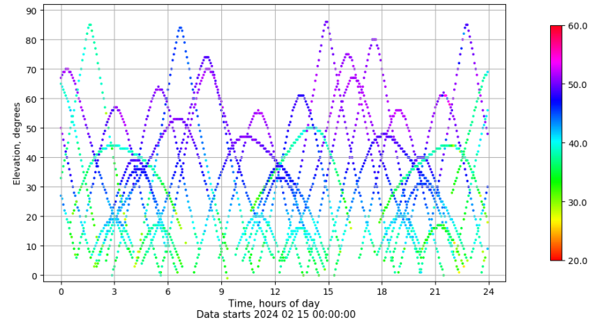
Time-elevation plot for station LALA. Signal to Noise S1C Data file LALA00ESP_R_2024046.xtr
