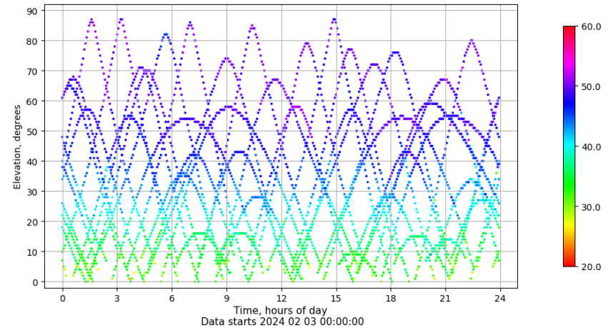
Time-elevation plot for station LALA. Signal to Noise S1C Data file LALA00ESP_R_2024034.xtr
