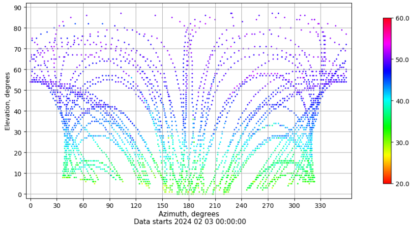
Azimuth-elevation plot for station LALA. Signal to Noise S1C Data file LALA00ESP_R_2024034.xtr
