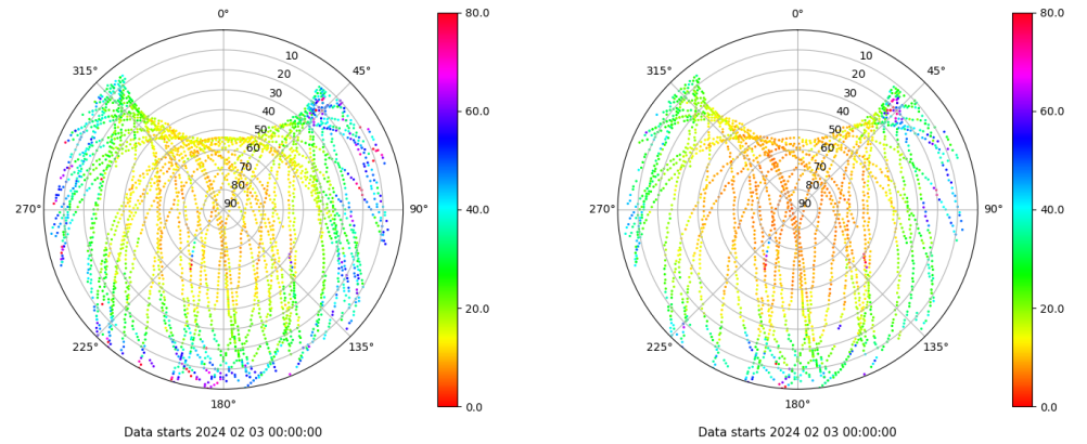
Skyplot for station LALA. Parameter M1C Data file LALA00ESP_R_2024034.xtr Skyplot for station LALA. Parameter M2X Data file LALA00ESP_R_2024034.xtr
