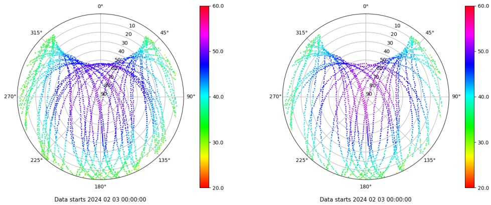
Skyplot for station LALA. Signal to Noise S1C Data file LALA00ESP_R_2024034.xtr Skyplot for station LALA. Signal to Noise S2X Data file LALA00ESP_R_2024034.xtr
