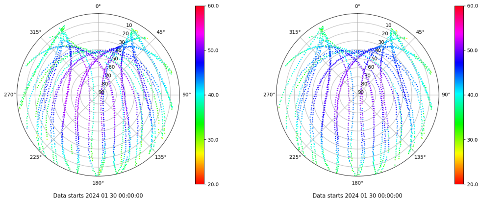
Skyplot for station LALA. Signal to Noise S1C Data file LALA00ESP_R_2024030.xtr Skyplot for station LALA. Signal to Noise S2C Data file LALA00ESP_R_2024030.xtr
