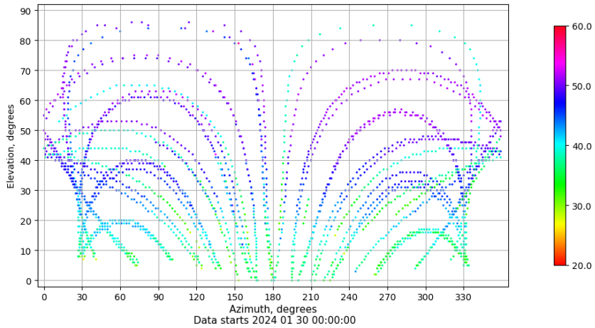
Azimuth-elevation plot for station LALA. Signal to Noise S1C Data file LALA00ESP_R_2024030.xtr
