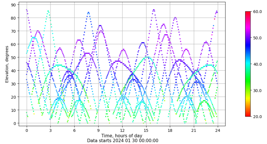
Time-elevation plot for station LALA. Signal to Noise S1C Data file LALA00ESP_R_2024030.xtr
