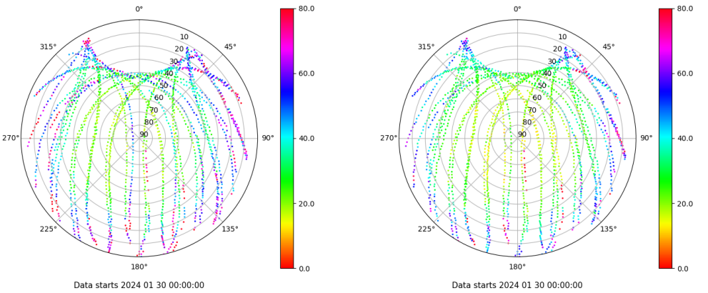
Skyplot for station LALA. Parameter M1C Data file LALA00ESP_R_2024030.xtr Skyplot for station LALA. Parameter M2C Data file LALA00ESP_R_2024030.xtr
