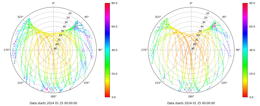
Skyplot for station LALA. Parameter M1C Data file LALA00ESP_R_2024025.xtr Skyplot for station LALA. Parameter M2X Data file LALA00ESP_R_2024025.xtr
