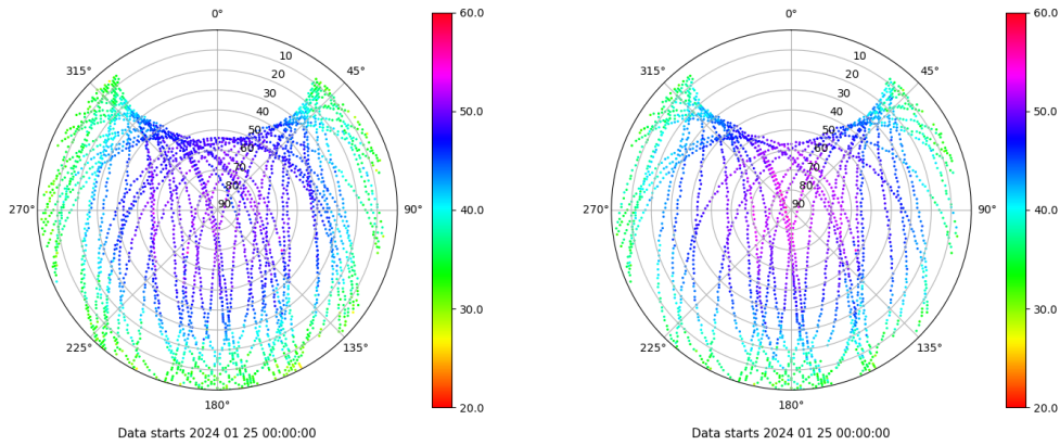
Skyplot for station LALA. Signal to Noise S1C Data file LALA00ESP_R_2024025.xtr Skyplot for station LALA. Signal to Noise S2X Data file LALA00ESP_R_2024025.xtr
