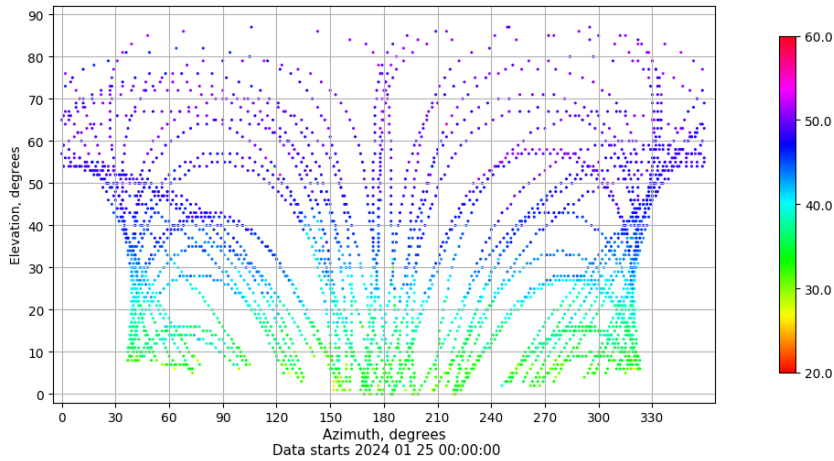
Azimuth-elevation plot for station LALA. Signal to Noise S1C Data file LALA00ESP_R_2024025.xtr
