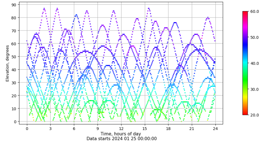
Time-elevation plot for station LALA. Signal to Noise S1C Data file LALA00ESP_R_2024025.xtr
