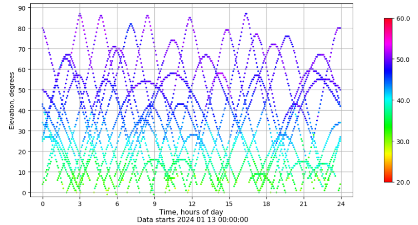
Time-elevation plot for station LALA. Signal to Noise S1C Data file LALA00ESP_R_2024013.xtr
