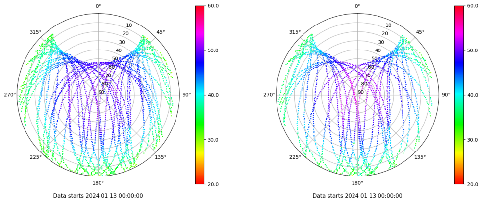
Skyplot for station LALA. Signal to Noise S1C Data file LALA00ESP_R_2024013.xtr Skyplot for station LALA. Signal to Noise S2X Data file LALA00ESP_R_2024013.xtr
