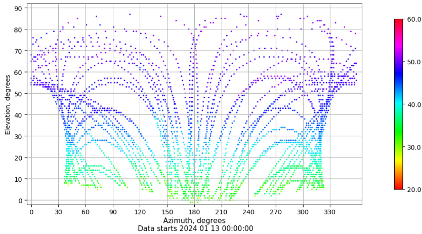
Azimuth-elevation plot for station LALA. Signal to Noise S1C Data file LALA00ESP_R_2024013.xtr
