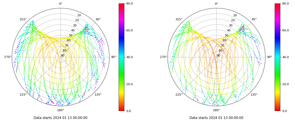
Skyplot for station LALA. Parameter M1C Data file LALA00ESP_R_2024013.xtr Skyplot for station LALA. Parameter M2X Data file LALA00ESP_R_2024013.xtr
