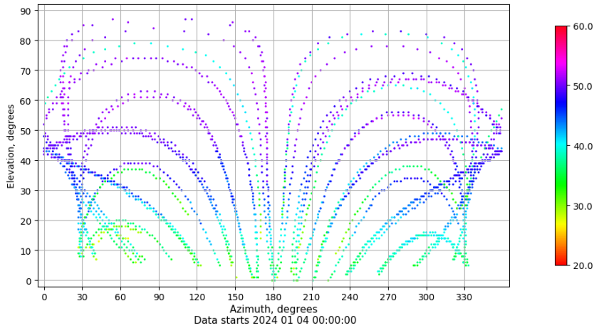
Azimuth-elevation plot for station LALA. Signal to Noise S1C Data file LALA00ESP_R_2024004.xtr
