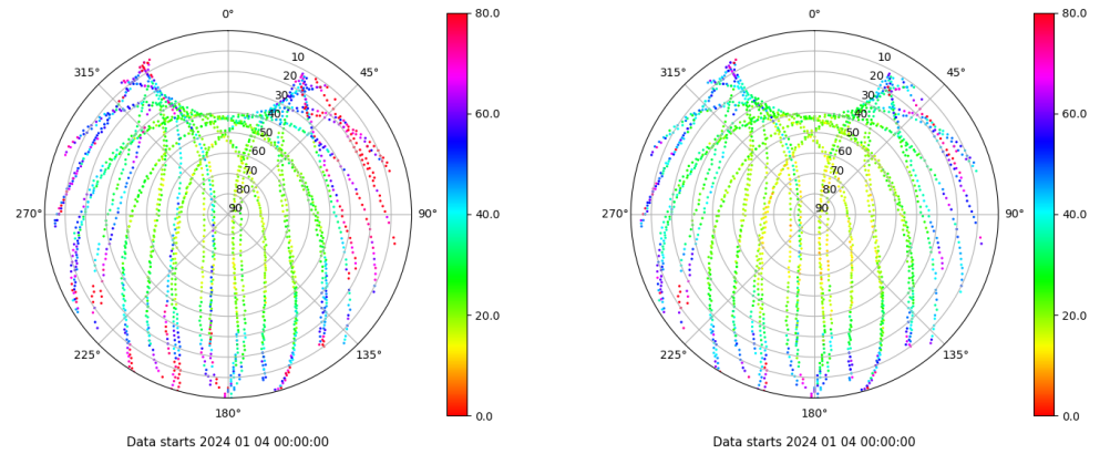
Skyplot for station LALA. Parameter M1C Data file LALA00ESP_R_2024004.xtr Skyplot for station LALA. Parameter M2C Data file LALA00ESP_R_2024004.xtr
