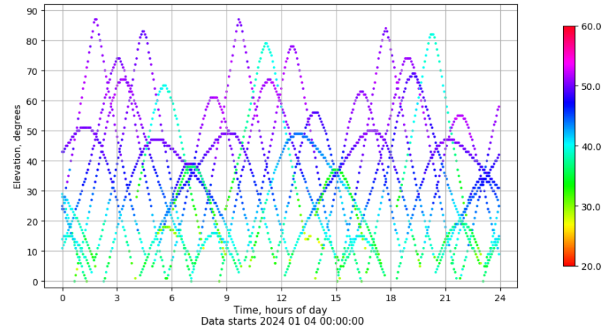
Time-elevation plot for station LALA. Signal to Noise S1C Data file LALA00ESP_R_2024004.xtr
