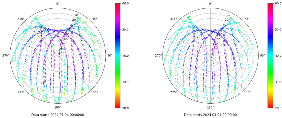
Skyplot for station LALA. Signal to Noise S1C Data file LALA00ESP_R_2024004.xtr Skyplot for station LALA. Signal to Noise S2C Data file LALA00ESP_R_2024004.xtr
