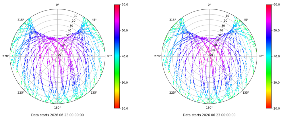
Skyplot for station IZAN. Signal to Noise S1C Data file IZAN00ESP_R_2026174.xtr Skyplot for station IZAN. Signal to Noise S2S Data file IZAN00ESP_R_2026174.xtr
