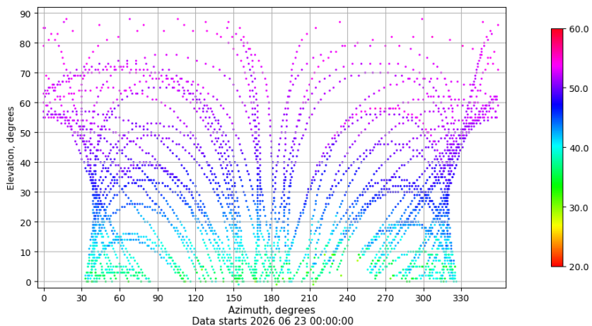
Azimuth-elevation plot for station IZAN. Signal to Noise S1C Data file IZAN00ESP_R_2026174.xtr
