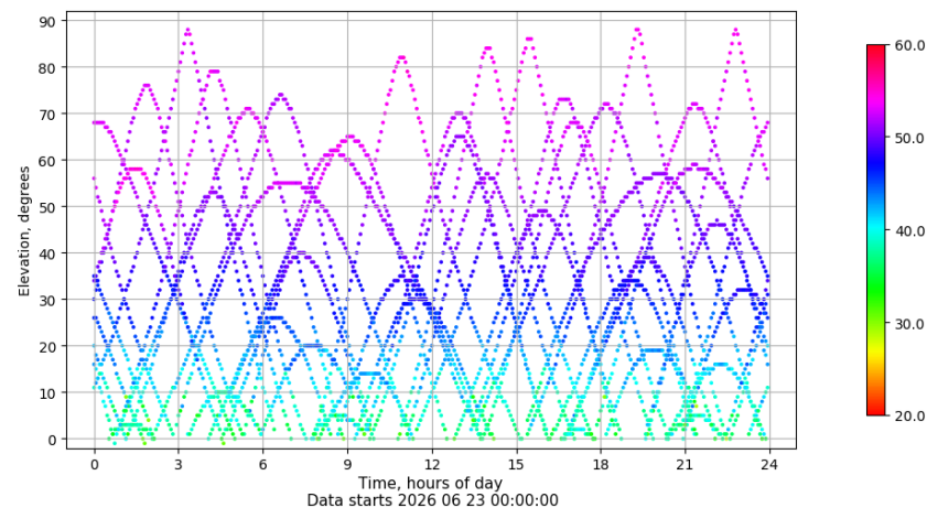
Time-elevation plot for station IZAN. Signal to Noise S1C Data file IZAN00ESP_R_2026174.xtr
