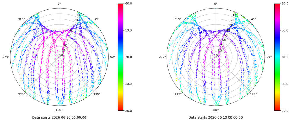
Skyplot for station IZAN. Signal to Noise S1C Data file IZAN00ESP_R_2026161.xtr Skyplot for station IZAN. Signal to Noise S2C Data file IZAN00ESP_R_2026161.xtr
