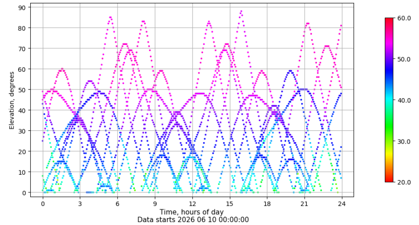
Time-elevation plot for station IZAN. Signal to Noise S1C Data file IZAN00ESP_R_2026161.xtr
