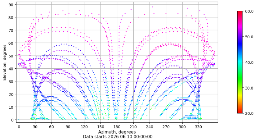
Azimuth-elevation plot for station IZAN. Signal to Noise S1C Data file IZAN00ESP_R_2026161.xtr
